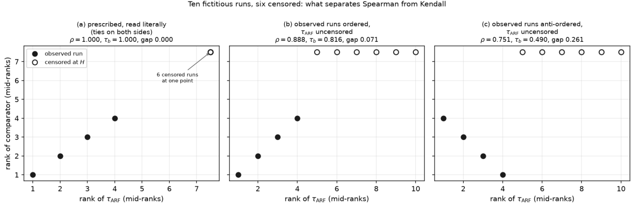
Figure 10. The three configurations of Table XVI, as mid-ranks. Filled markers: observed runs; hollow markers: runs censored at H , which share one mid-rank on the comparator side. (a) Tying the six censored runs on the \tau_{\text{ARF}} side as well makes the two coefficients coincide. (b) With \tau_{\text{ARF}} left uncensored, the same four ordered observations already separate Spearman from Kendall by 0.071. (c) Anti-ordering the four observations widens the gap to 0.261. Table QCD_contre_exemple_kendall.
