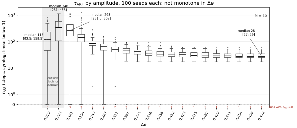
Figure 9. \tau_{\text{ARF}} on the 100 seeds of each amplitude; the four medians of Table XV are annotated with their interval. The axis is symmetric logarithmic, linear below 1: a plain logarithmic axis would silently drop the 34 runs in which a tree is replaced at the change point itself ( \tau_{\text{ARF}} = 0 ), and the box would rest on 97 to 99 seeds while the title claims 100. Their count per amplitude is written in red on the zero line; they occur at all 20 amplitudes, three at the lowest and one at the highest. What to see: the median rises from the first amplitude to the second before it falls, the spread shrinks by more than an order of magnitude across the grid, and the two shaded amplitudes lie outside the decision domain.
