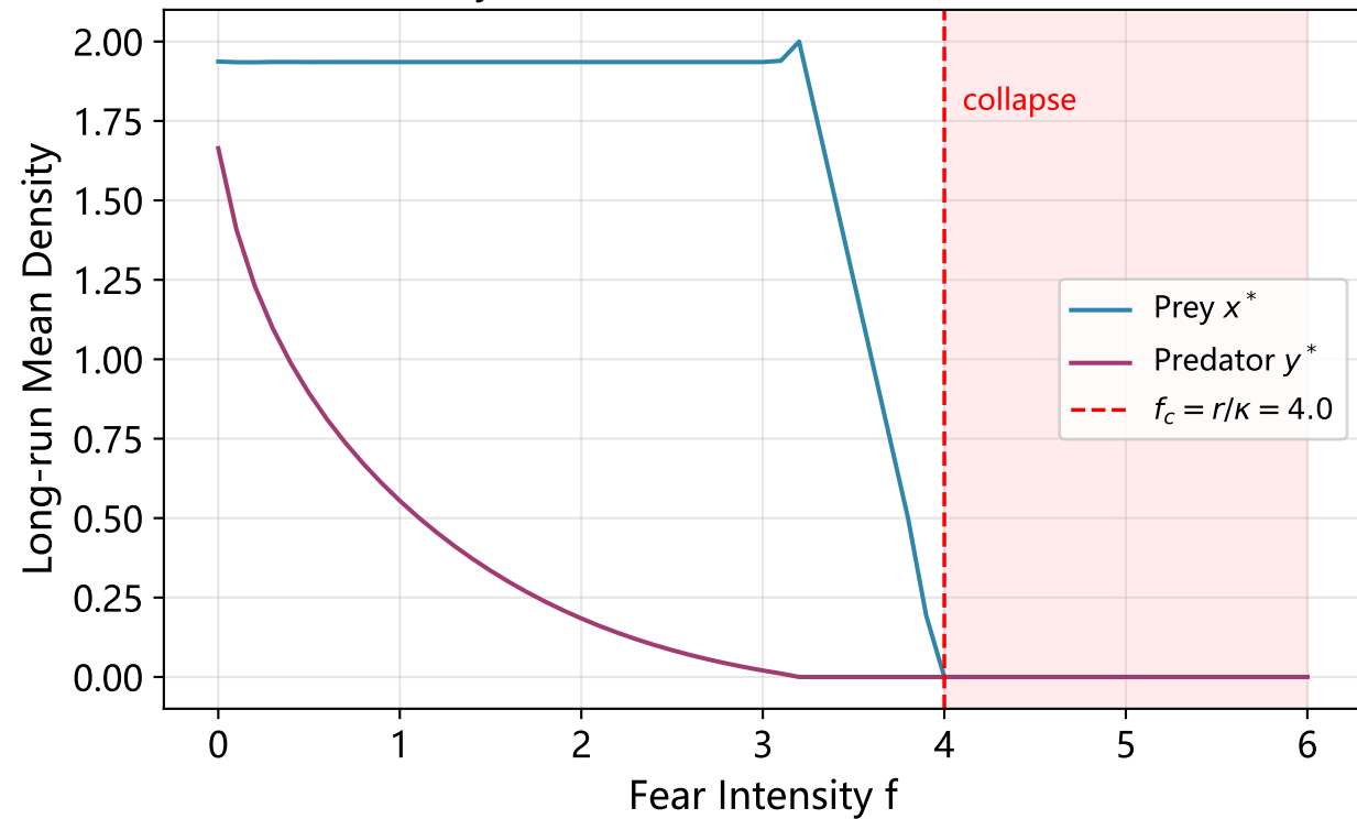
Steady State vs Fear (cost-of-fear model)
