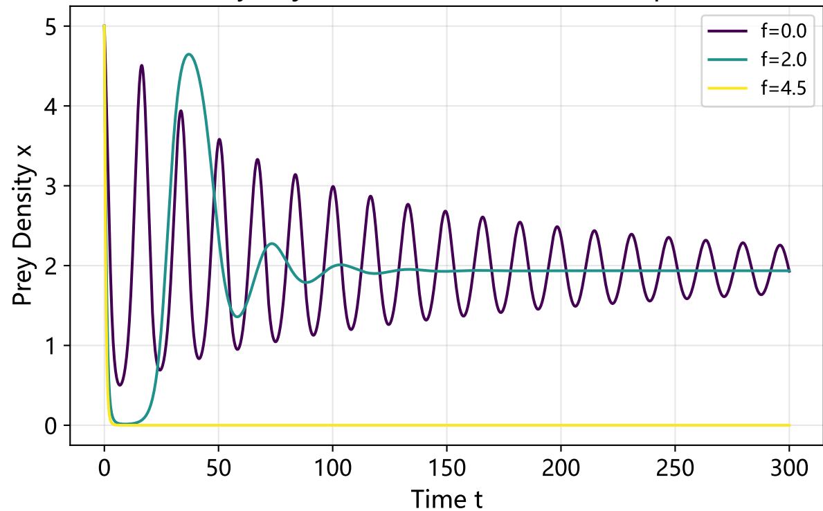
Prey Trajectories: Persistence vs Collapse
