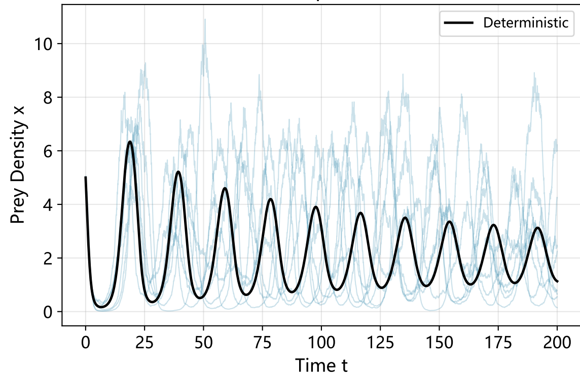
Stochastic Sample Paths ( f=1.0 )
