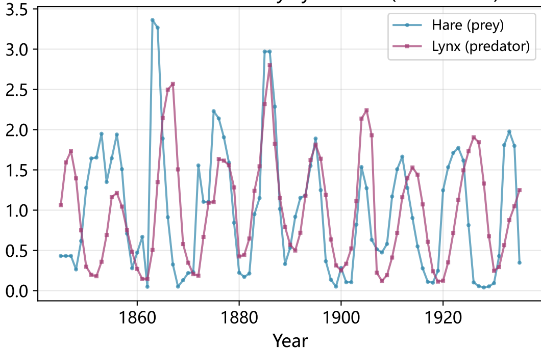
Real Data: Hudson Bay Lynx-Hare (1845-1935)
