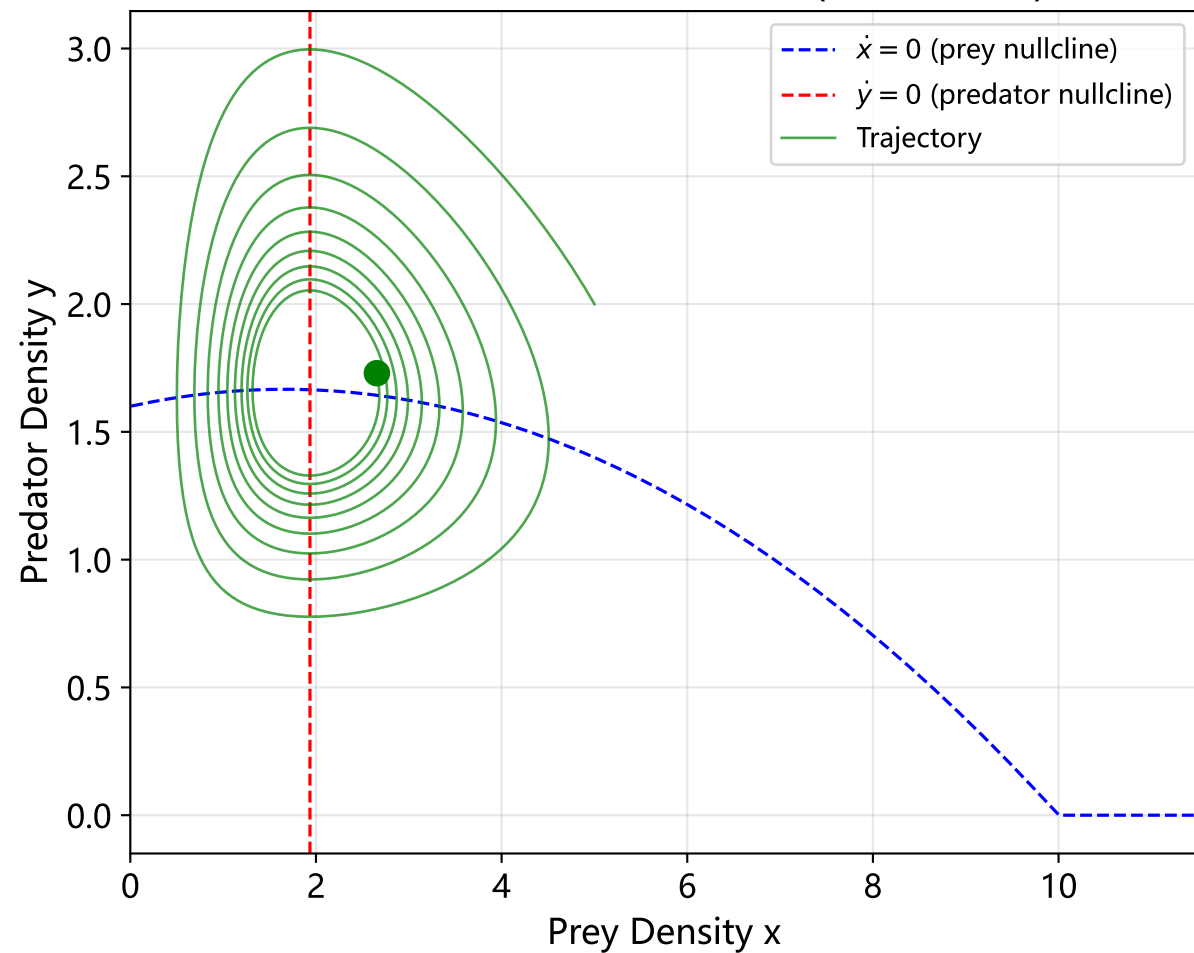
Phase Portrait with Nullclines (Base Model)
