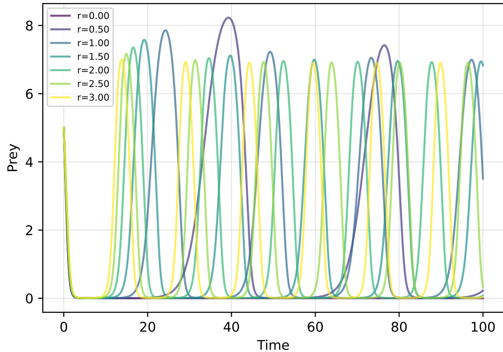
Prey — r sweep
