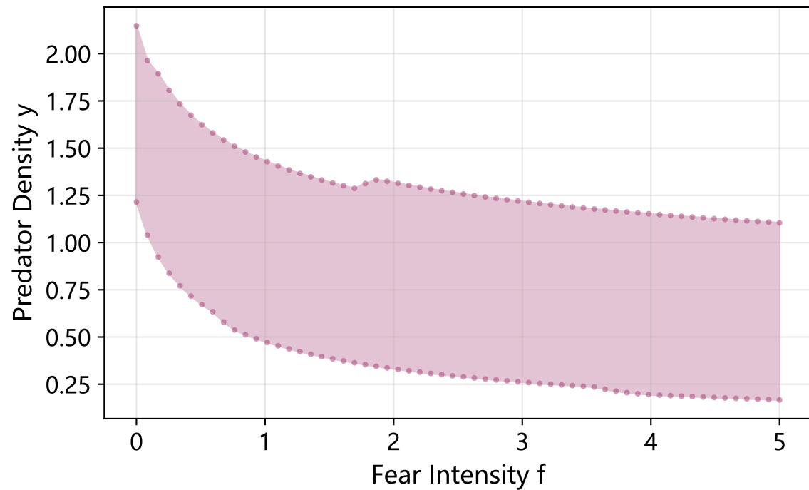
Predator Extrema
