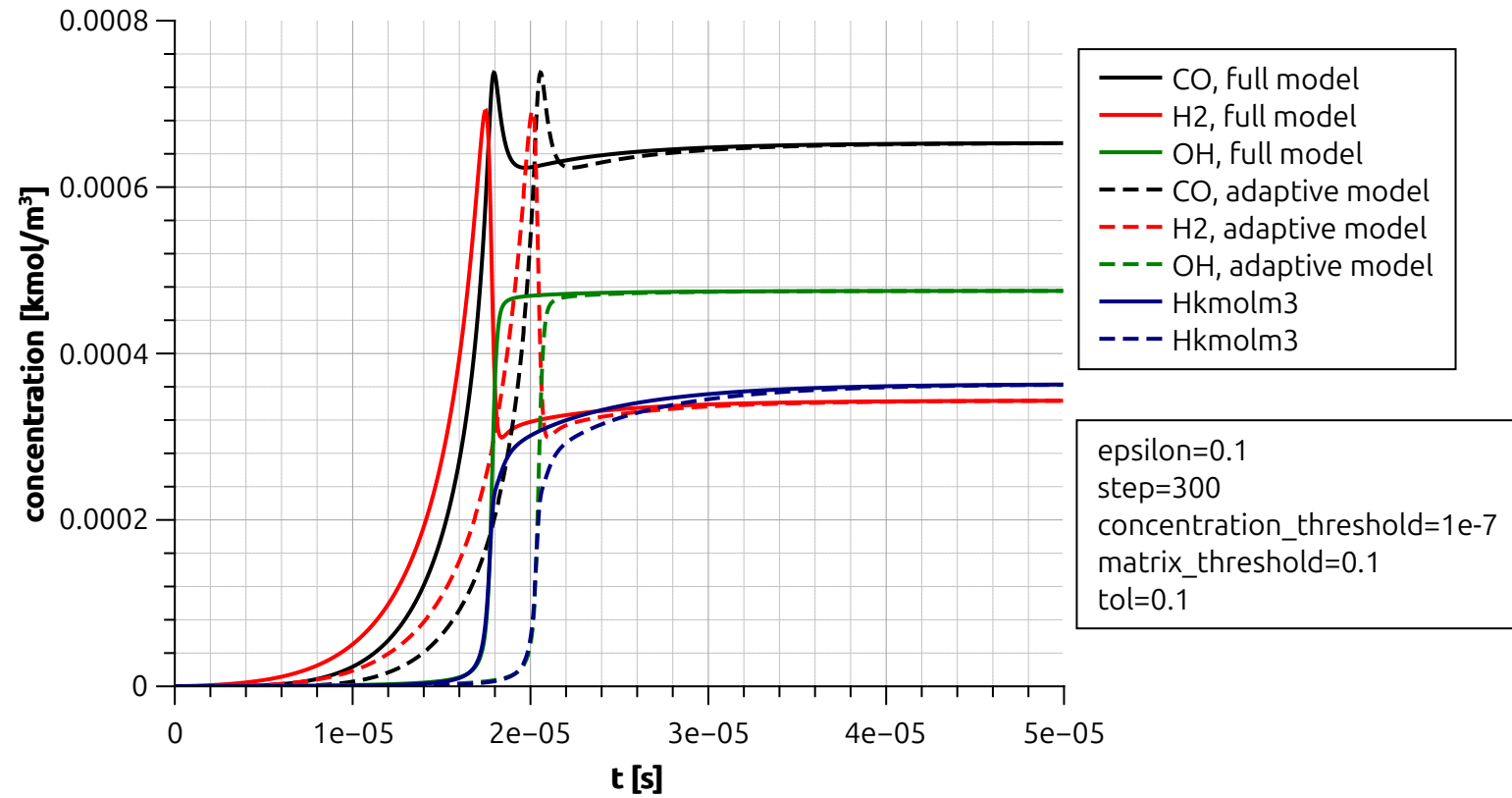
adaptive vs full model, constant pressure
