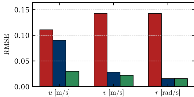
Velocity RMSE Comparison
