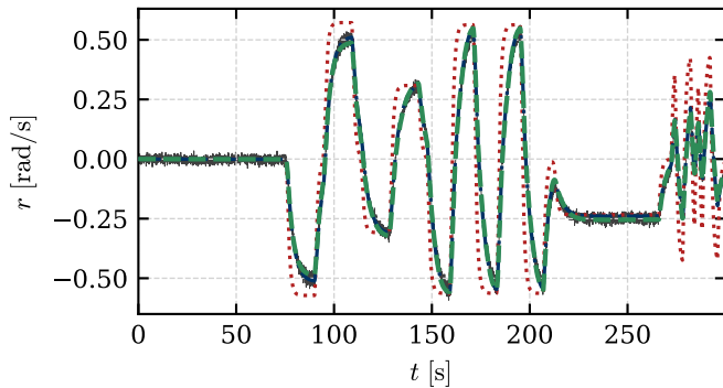
Yaw Rate r(t)
