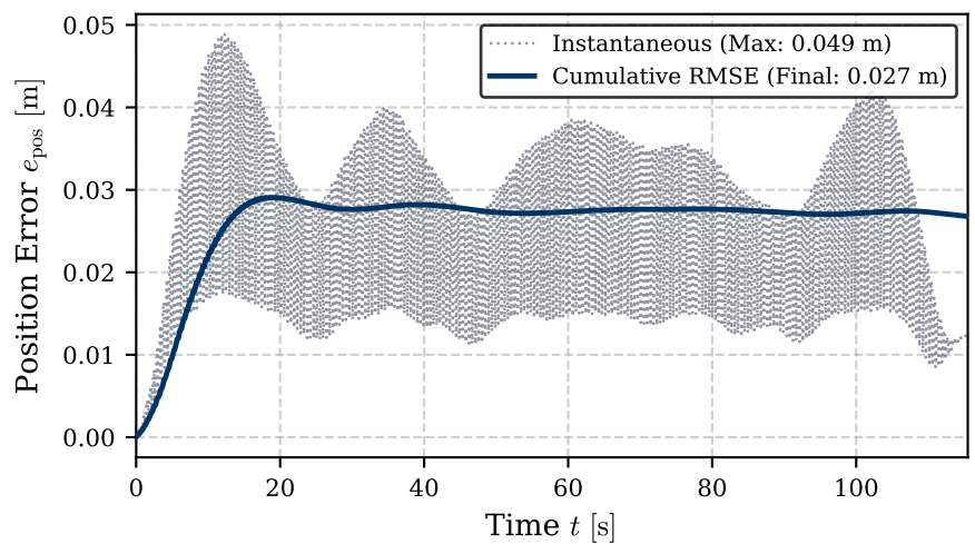
Case 3 (6-Param NLP Flatness-MPC, N=30) - Real-Time Control &amp; Computing Performance
