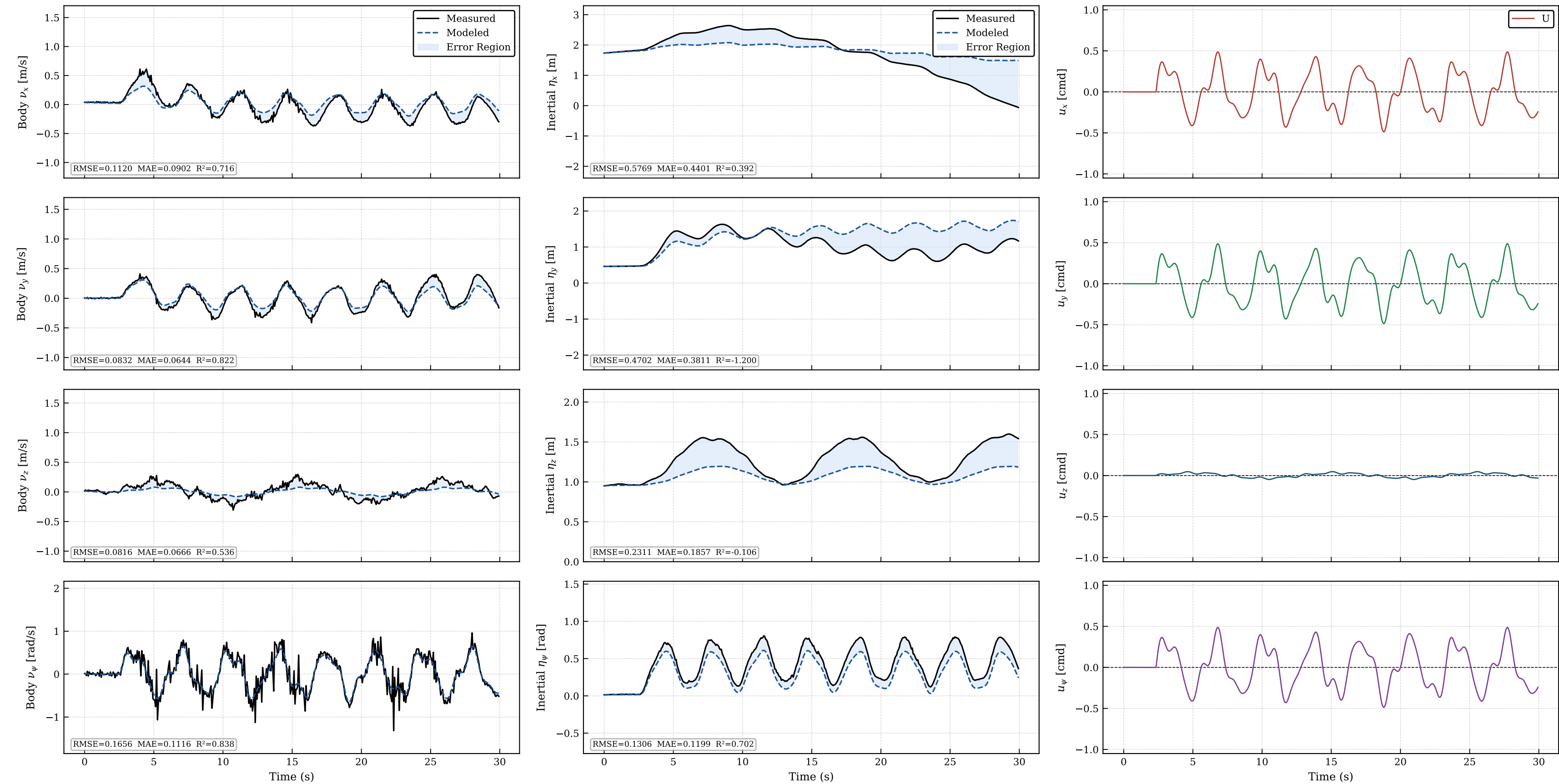
Validation — coupled_sine_ud_all_08_Aug_2026_17h15min_B10_15Hz_COMPLETEO.csv
