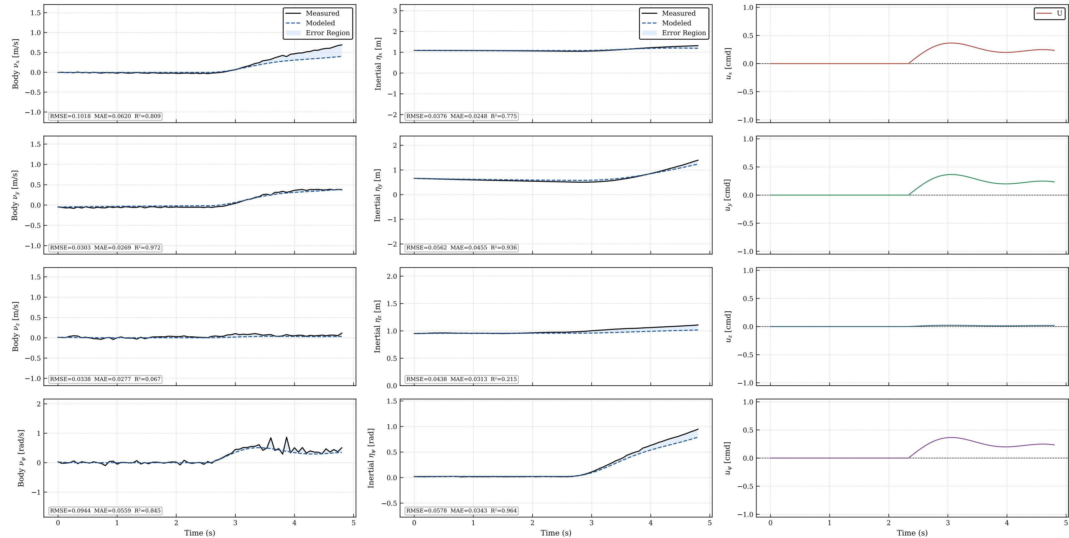
Validation — coupled_sine_ud_all_08_Aug_2026_17h12min_B10_15Hz_COMPLETEO.csv
