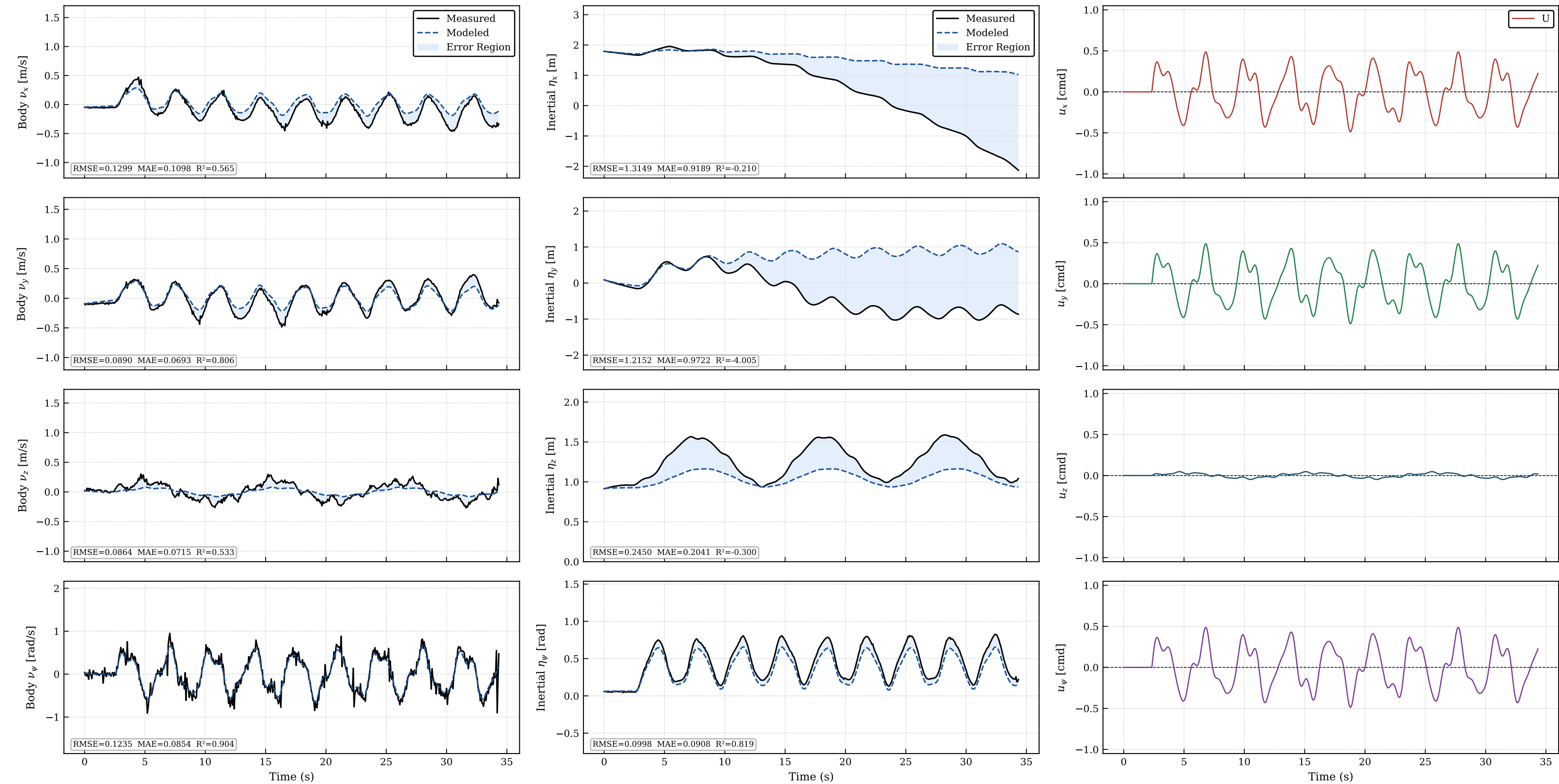
Validation — coupled_sine_ud_all_08_Aug_2026_17h14min_B10_15Hz_COMPLETEO.csv
