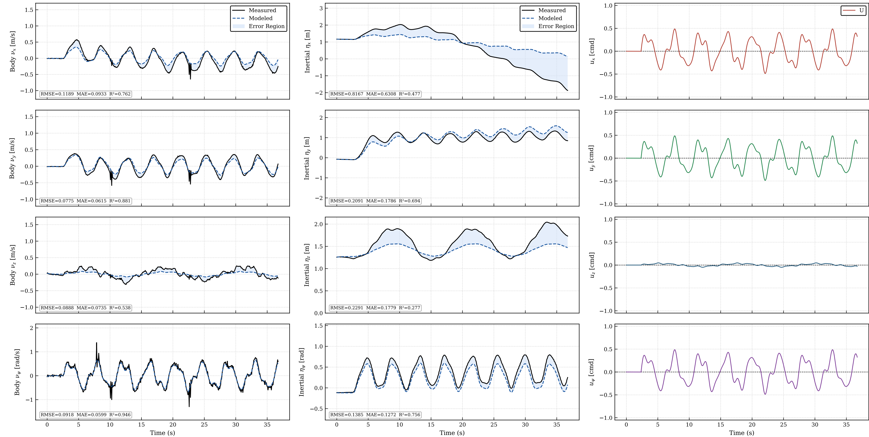
Validation — coupled_sine_ud_all_09_Aug_2026_11h40min_B10_15Hz_COMPLETEO.csv
