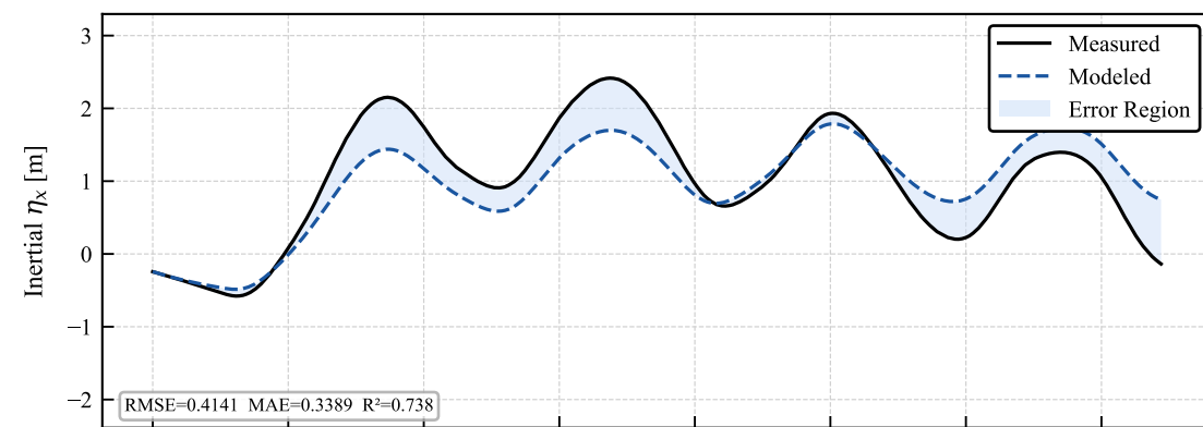
Validation — uncoupled_sine_udTheta_08_Aug_2026_16h39min_B10_15Hz_COMPLETEO.csv
