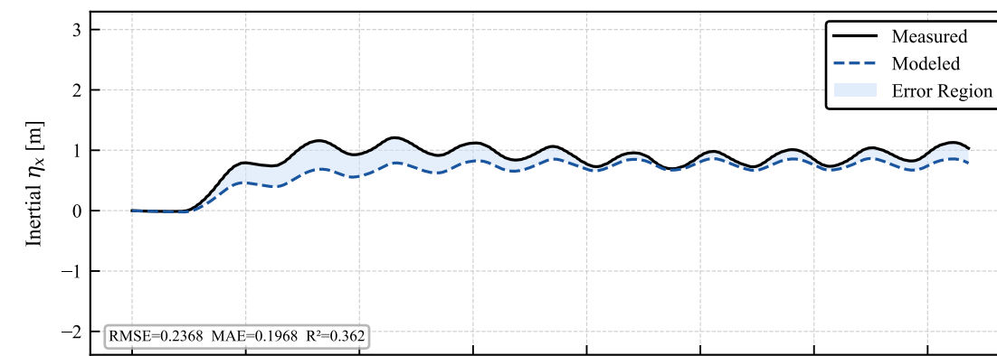
Validation — uncoupled_sine_udTheta_09_Aug_2026_11h10min_B10_15Hz_COMPLETEO.csv
