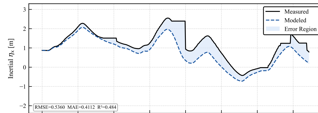
Validation — coupled_sine_joystick_09_Aug_2026_11h46min_B10_15Hz_COMPLETEO.csv
