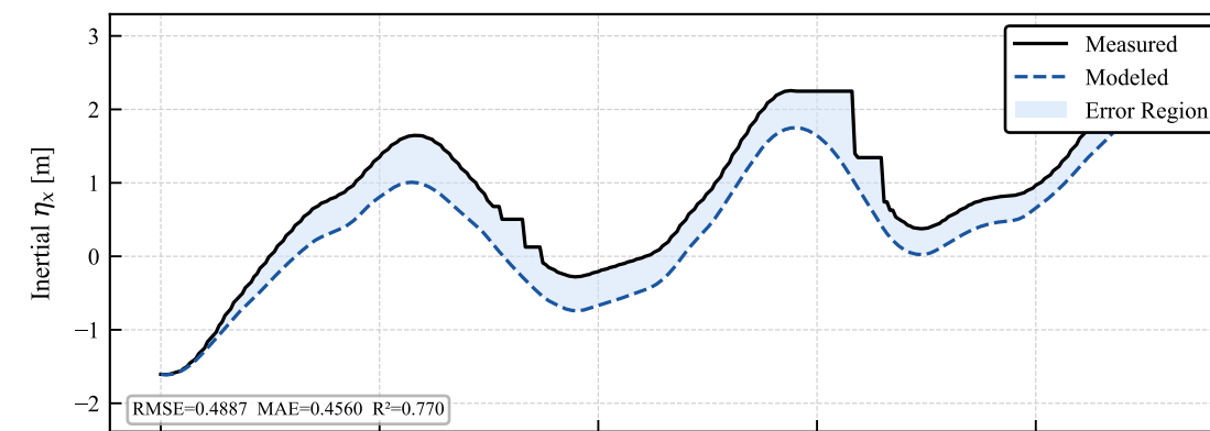
Validation — coupled_sine_joystick_09_Aug_2026_11h44min_B10_15Hz_COMPLETEO.csv
