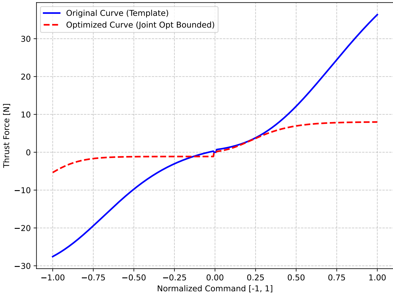
T200 Thruster Command vs. Thrust Force (9-param model)
