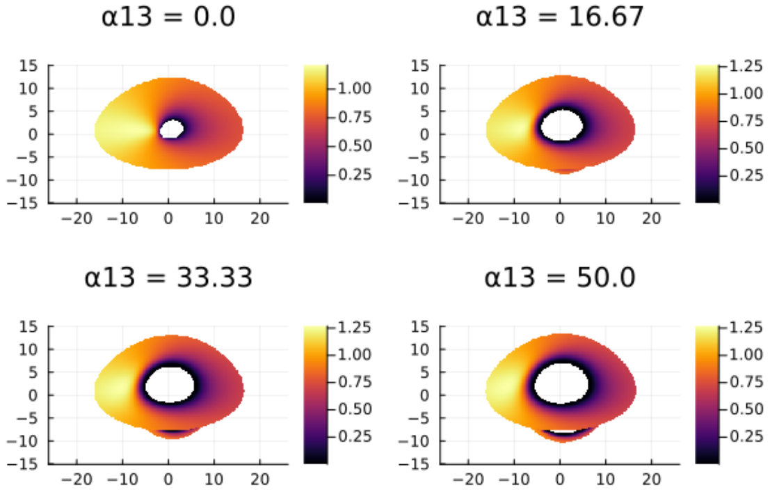
Figure 3.7: The effect of \alpha_{13} on the accretion disk render. The event horizon appears to grow with \alpha_{13}
