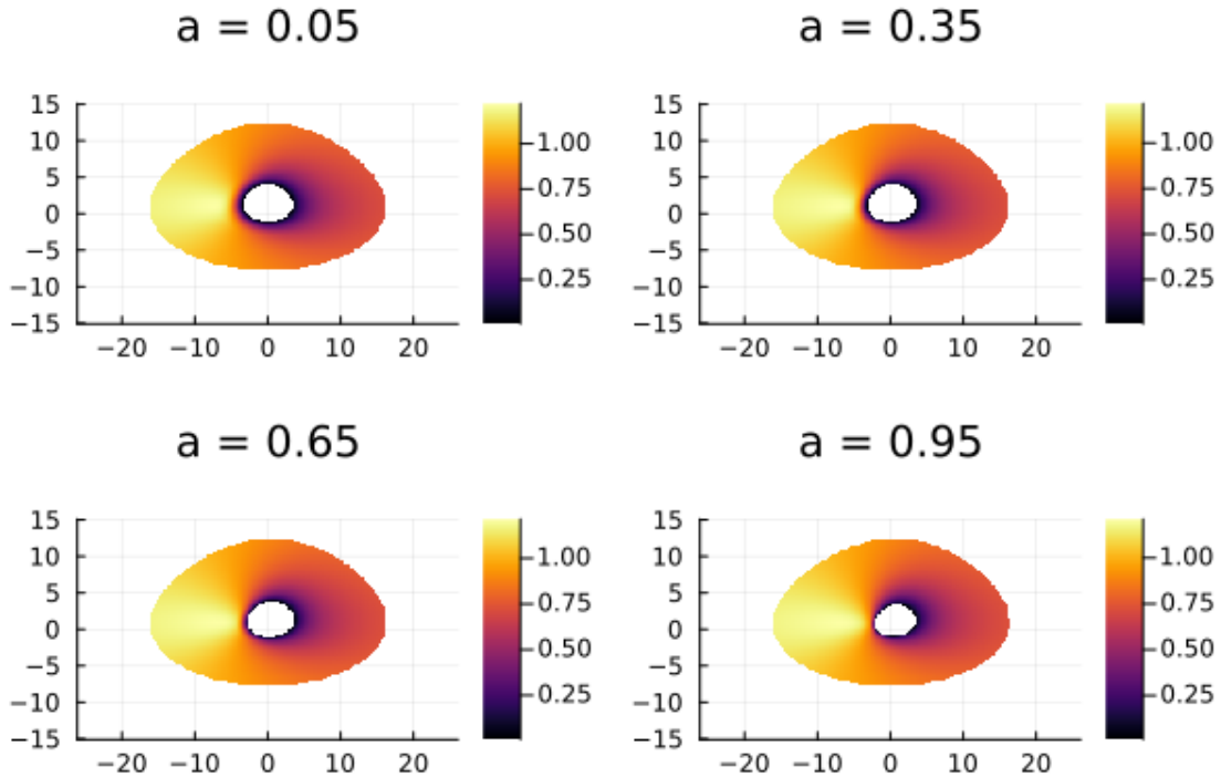
Figure 3.10: The effect of black hole spin on the redshift image. The event horizon appears to shrink.
