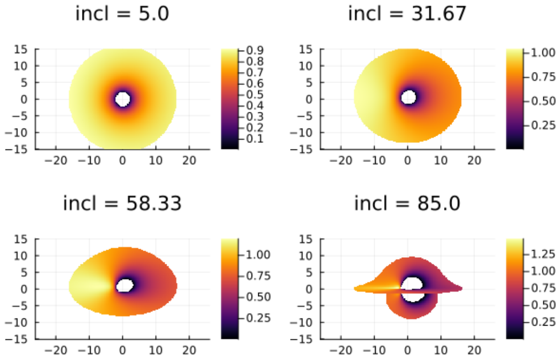
Figure 3.9: The effect of inclination on the redshift image. The redshift becomes more apparent as the inclination increases and the disk becomes edge on. This agrees with the observed line profile trend of energy increasing with inclination as the effects of doppler shifting become more apparent with increasing energy.
