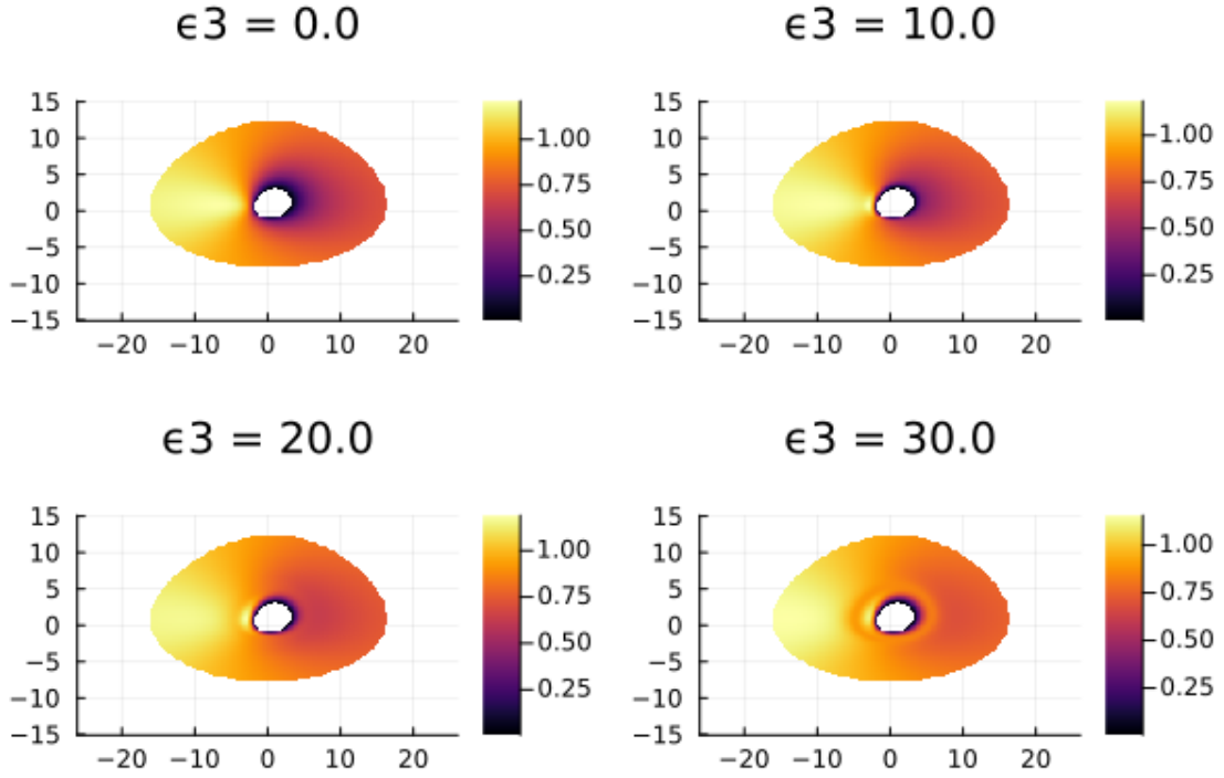
Figure 3.8: The effect of \epsilon_3 on the redshift image. The shape of the disk does not change but the redshift profile does, particularly in the inner regions where the redshift tends to increase.
