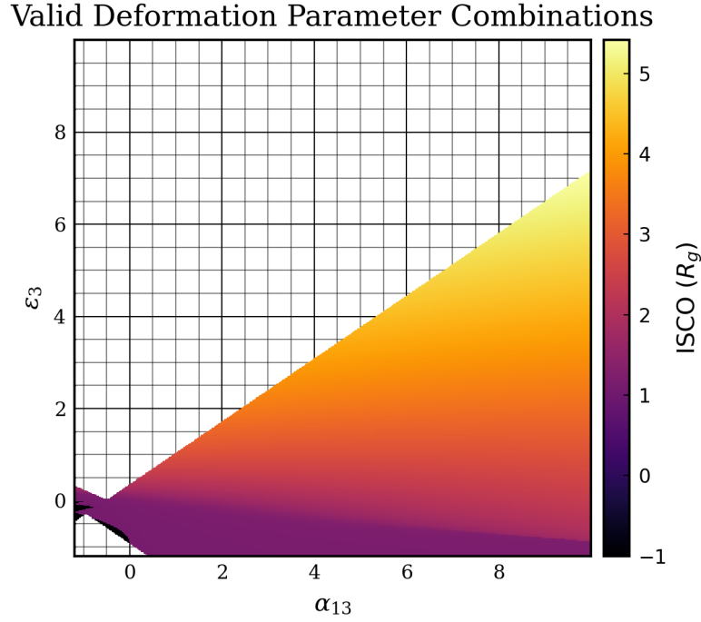
Figure 8.1: The valid deformation parameters for a maximally spinning ( a = 0.998 ) black hole. The unshaded regions show where a naked singularity would be present, and the black regions show where there is not an ISCO.
