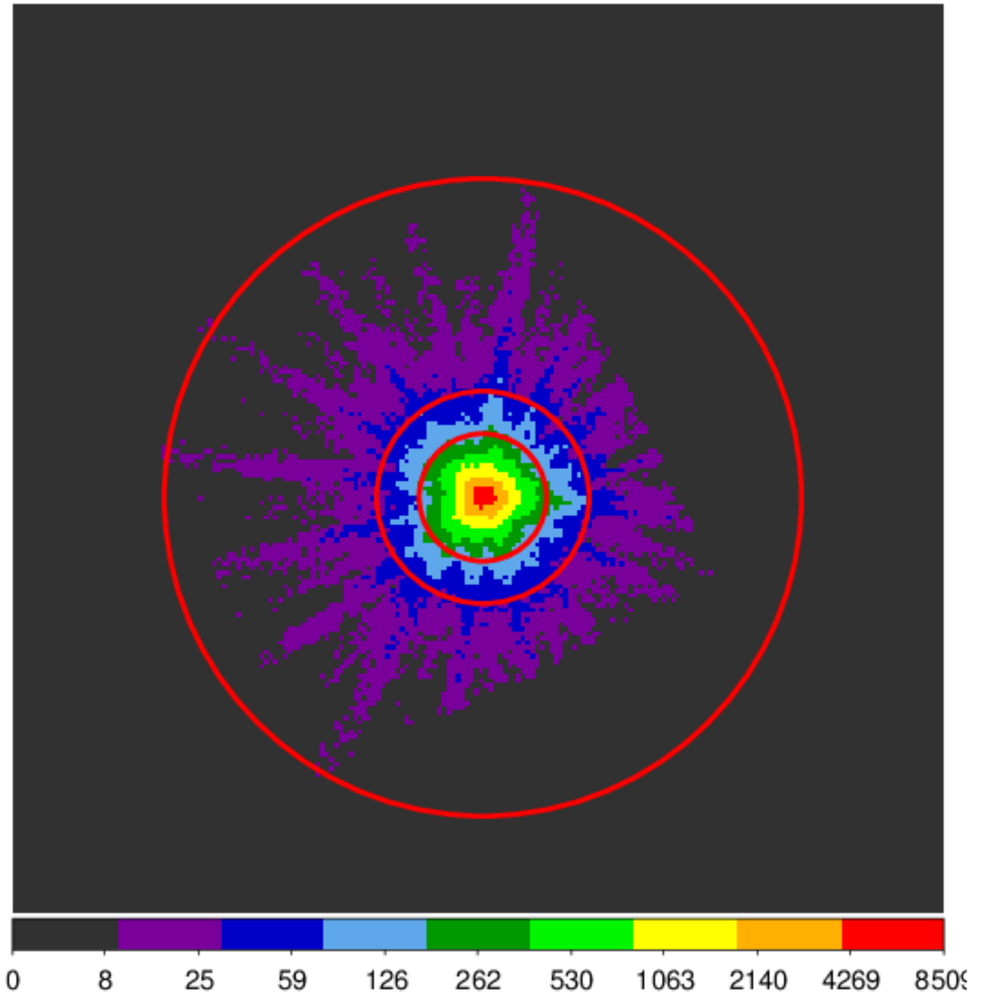
Figure 2.1: The regions used for spectrum extraction. The outer two circles were used to select an annulus for the background. The inner circle was used for the source region. The regions were centered at (25631.2,23903,300) with radii of 300, 500, and 1500 pixels.
