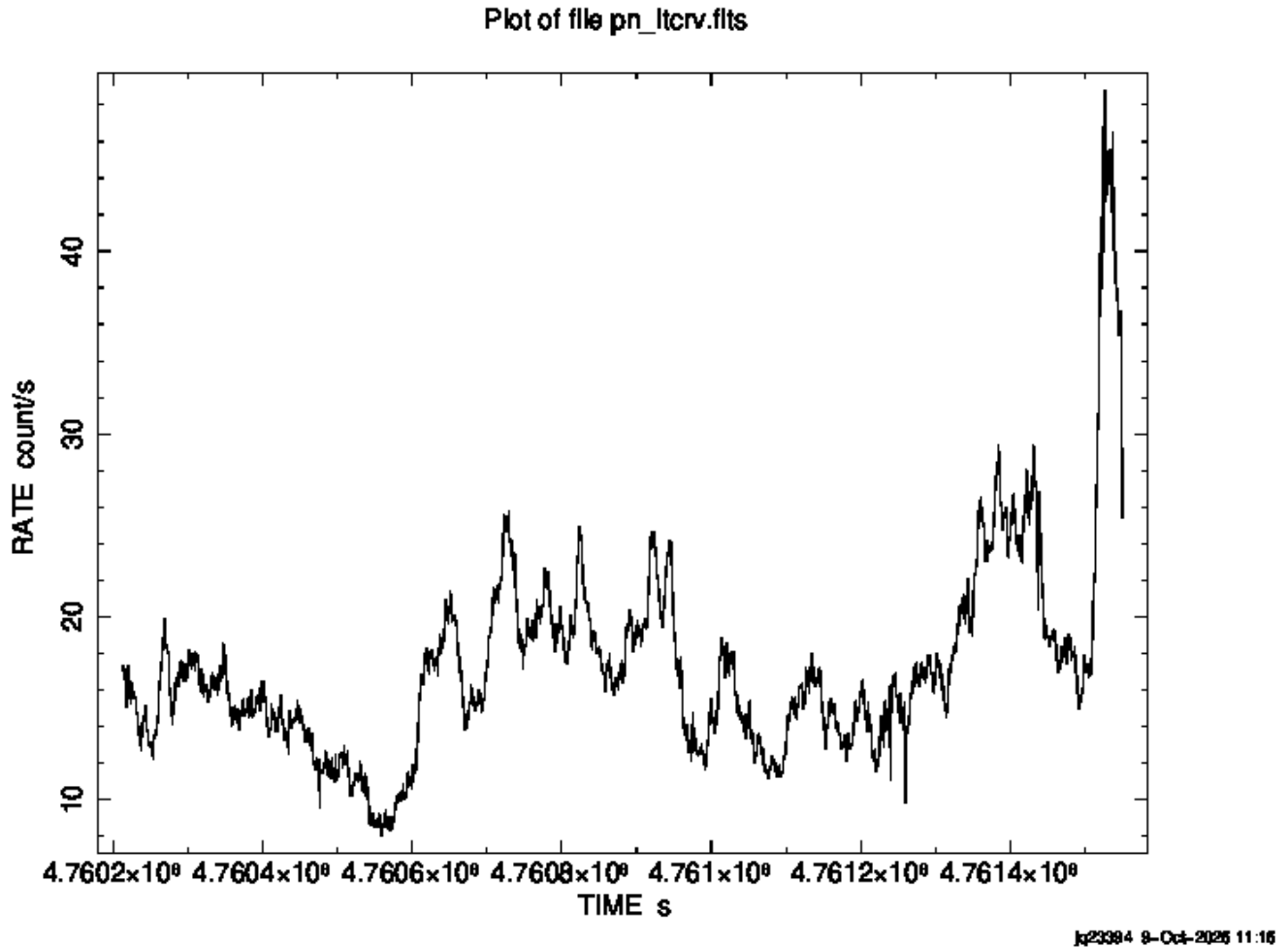
Figure 3.1: The pn lightcurve of the observation. A large flare is again observed at the end of the observation, which was filtered out from the data analysis.
