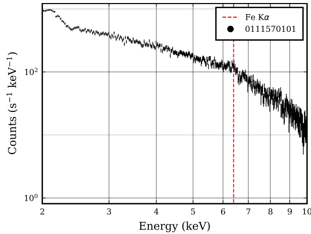
Figure 3.4: The spectrum from obsid 0111570101. The data was once again plotted with ViewSpectrum.jl
