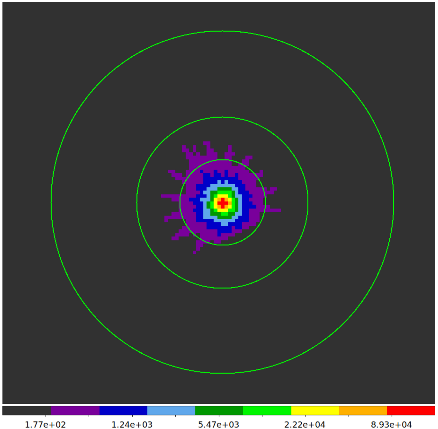
Figure 3.2: The regions selected for source and background extraction. The scale at the bottom denotes how many events were detected in each pixel.
