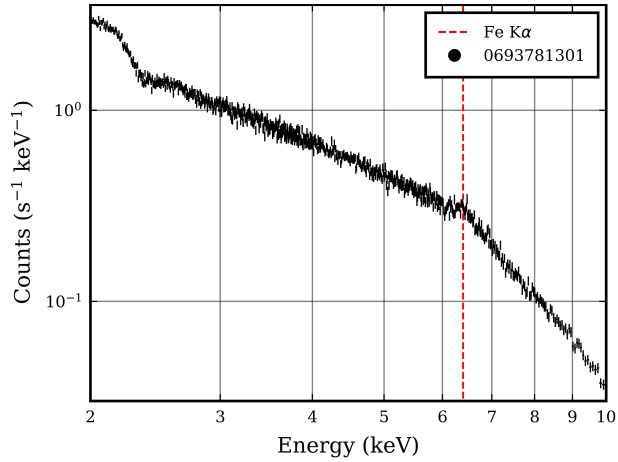
Figure 3.3: The pn spectrum of MCG-6-30-15 from observation ID 0693781301, regrouped to have at least 400 counts per bin. The red line marks 6.4 keV where the Fe K\alpha emission line is expected. A bump is observed in the expected region.
