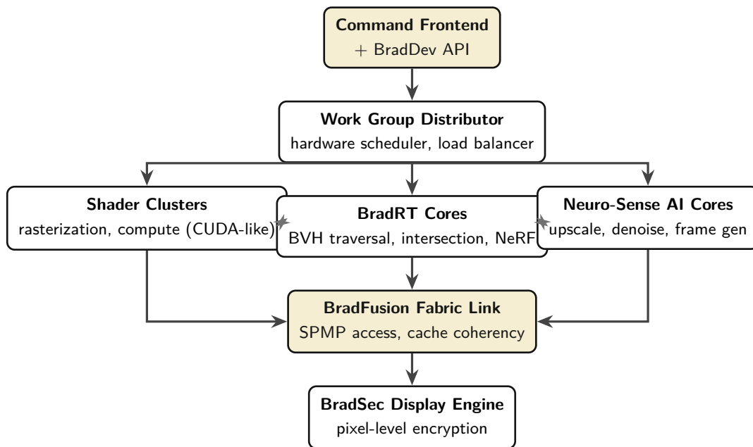
Figure 1: Gen1 unified GPU architecture — BRADGFX / BRADFX
