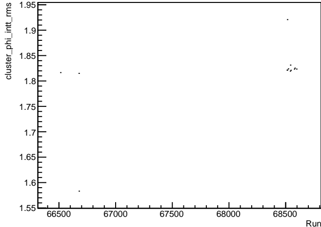
cluster_phi_intt_rms
