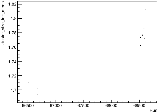
cluster_size_intt_mean
