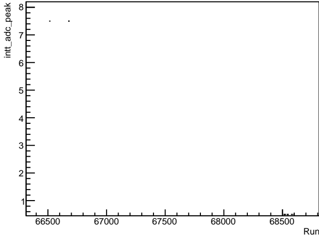
intt_adc_peak
