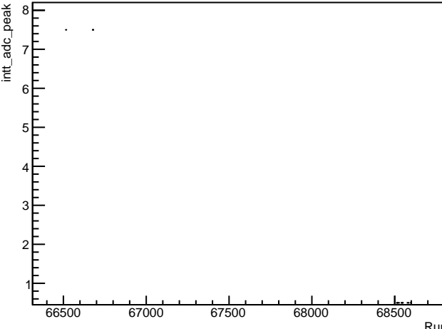
intt_adc_peak
