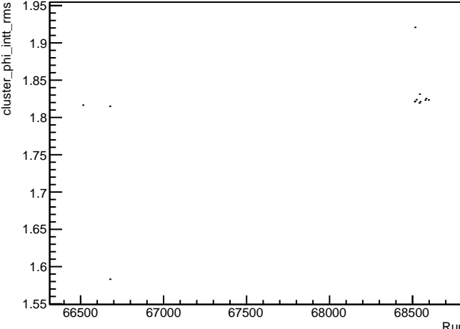
cluster_phi_intt_rms
