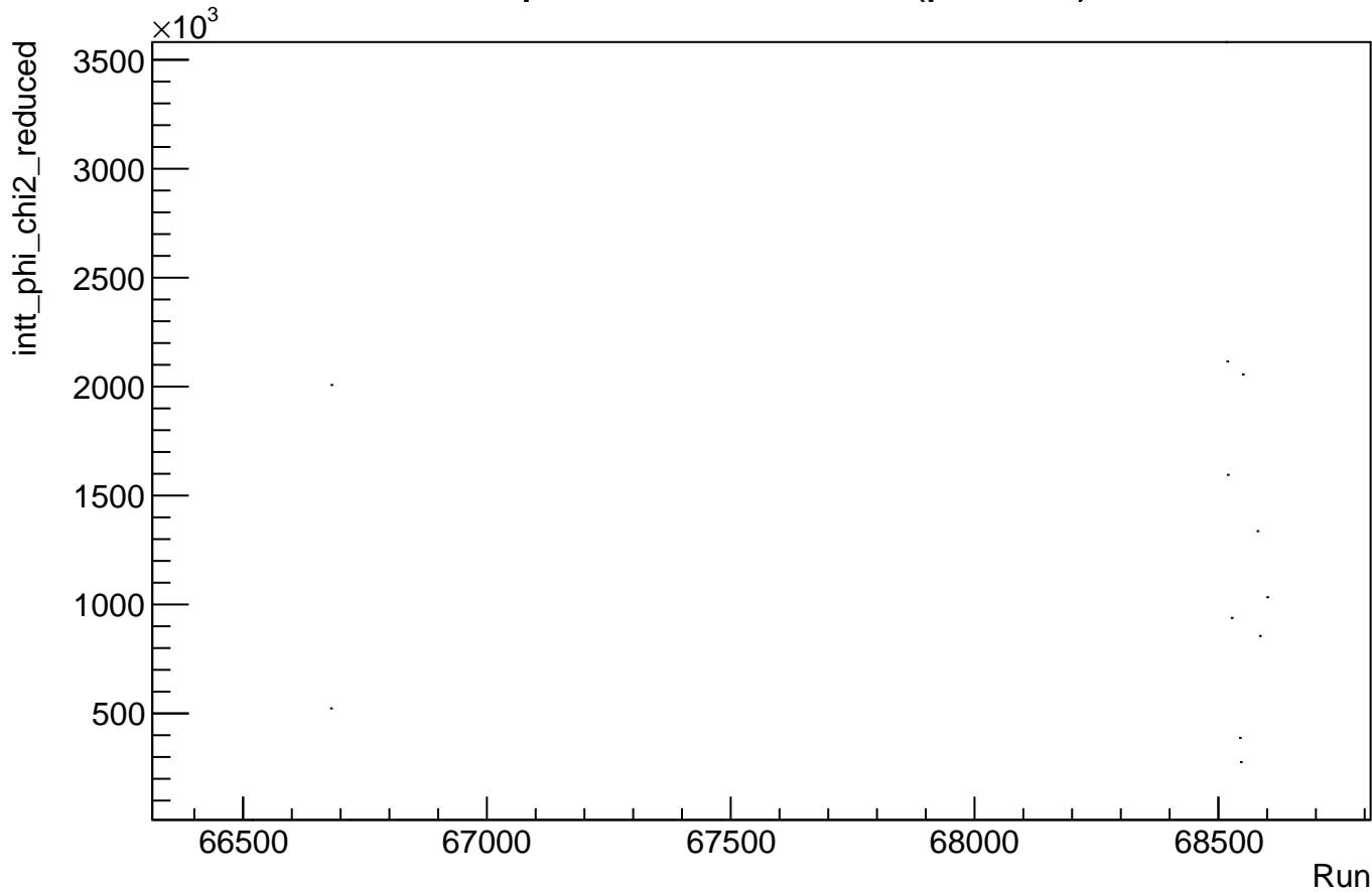
intt_phi_chi2_reduced (per run)
