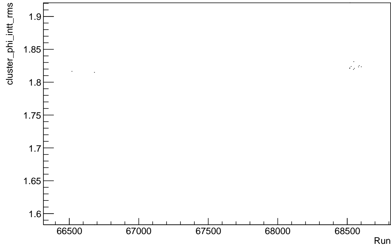
cluster_phi_intt_rms (per run)
