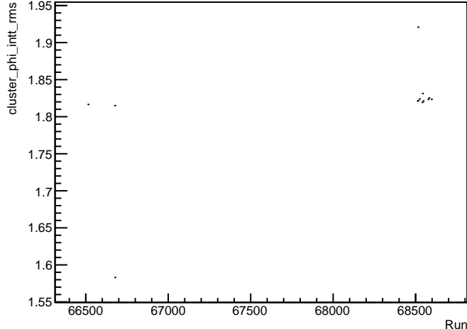
cluster_phi_intt_rms
