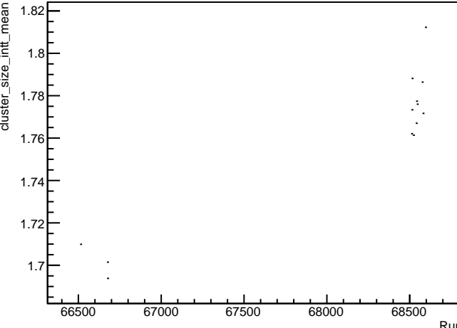
cluster_size_intt_mean
