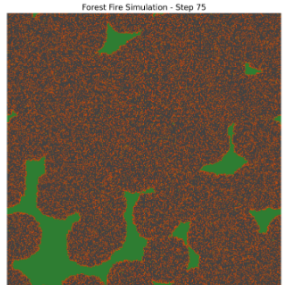
Fig. 7. Step 75: Late propagation stage. Most of the domain is burned; surviving vegetation is confined to isolated islands protected by burned firebreaks.
