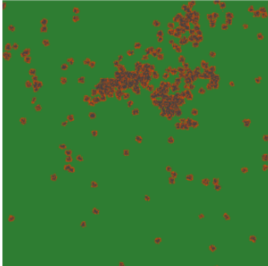
Fig. 5. Step 10: Early expansion phase. Independent fire clusters grow outward from FIRMS hotspot locations; most of the domain remains vegetated (green).
