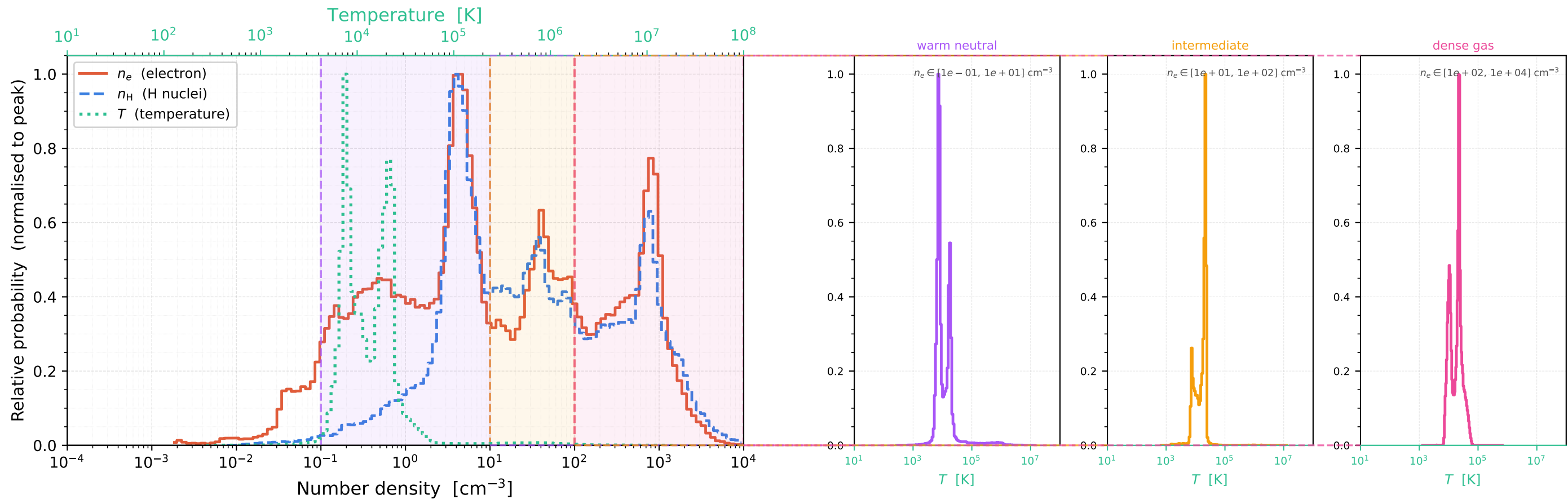
Number Density and Temperature PDFs (200 pc sphere region)
