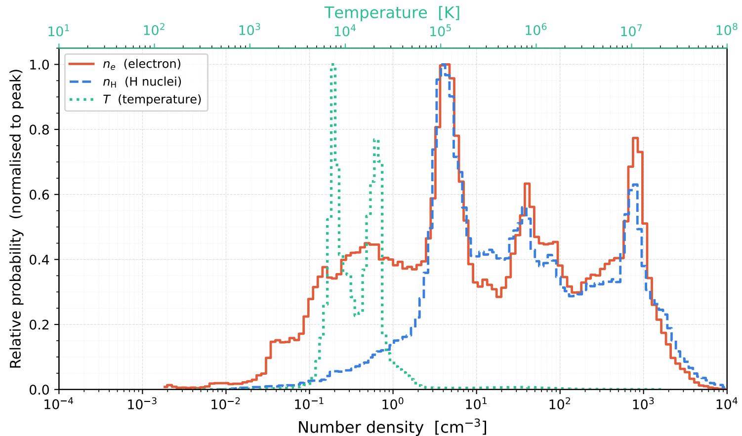
Number Density and Temperature PDFs (200 pc sphere region)
