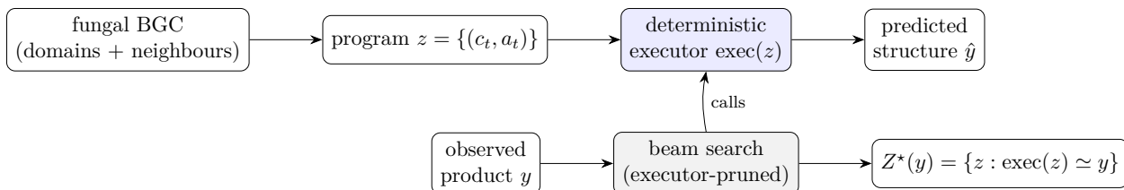
Figure 1: The executor (top) renders a program to a structure; the verifier (bottom) inverts it by beam-searching programs, executing each candidate and pruning any whose partial product cannot reach y , returning the exact consistent set Z^*(y) .
