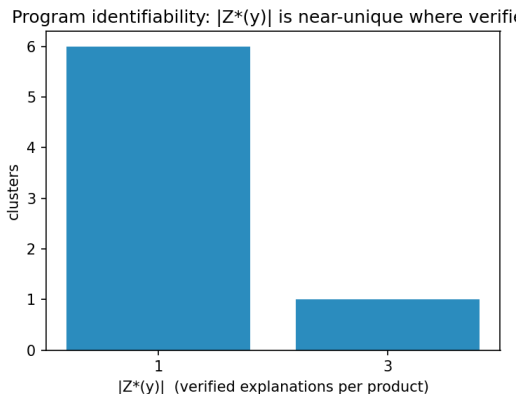
Figure 4: Explanation multiplicity for the seven tailoring-latent-verified clusters: six are uniquely explained and one has three consistent explanations. Where the joint search succeeds it is near-unique—the regime in which a verifier-constrained objective is well posed.
