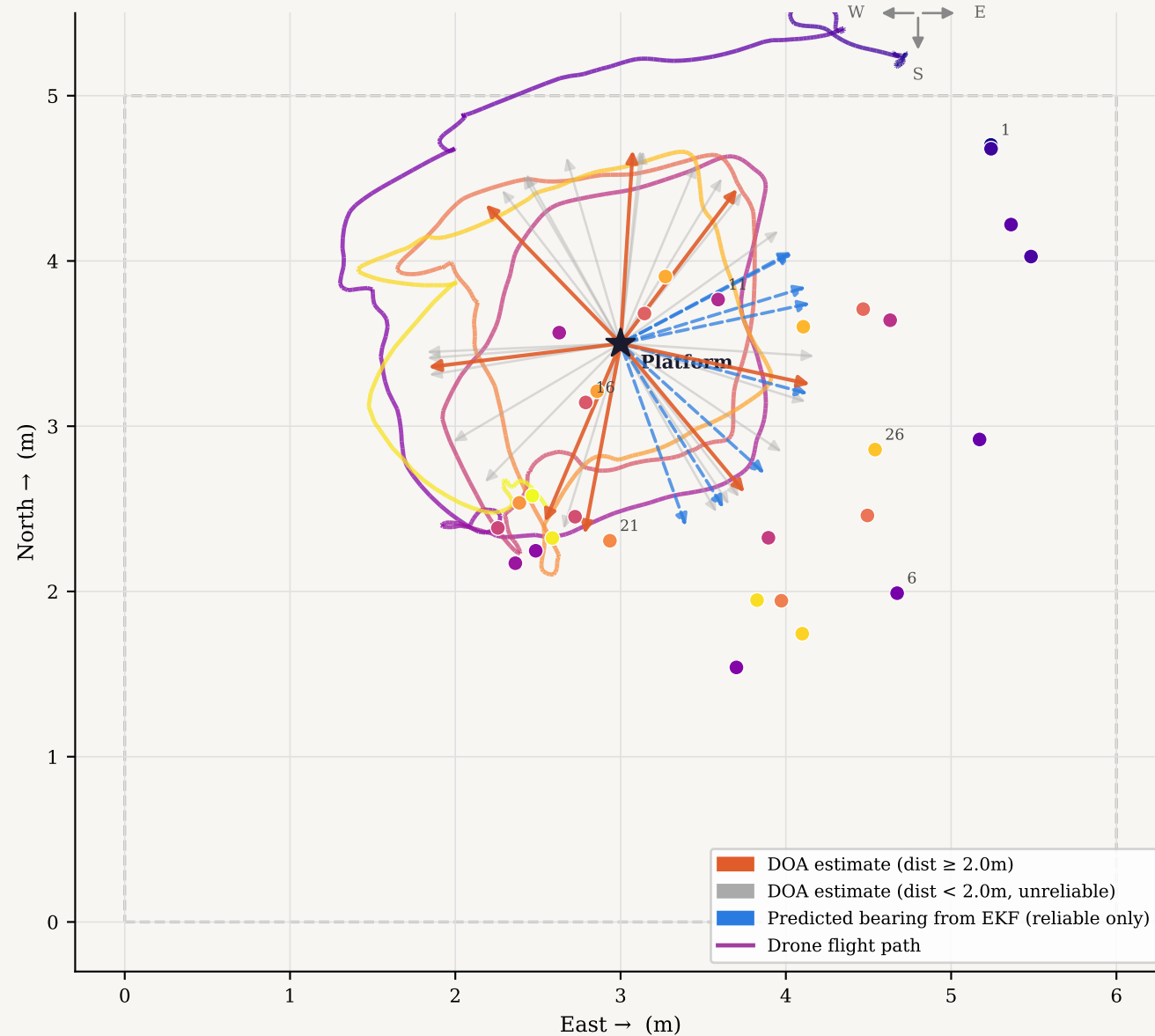
Top-down view: flight path & DOA estimates
