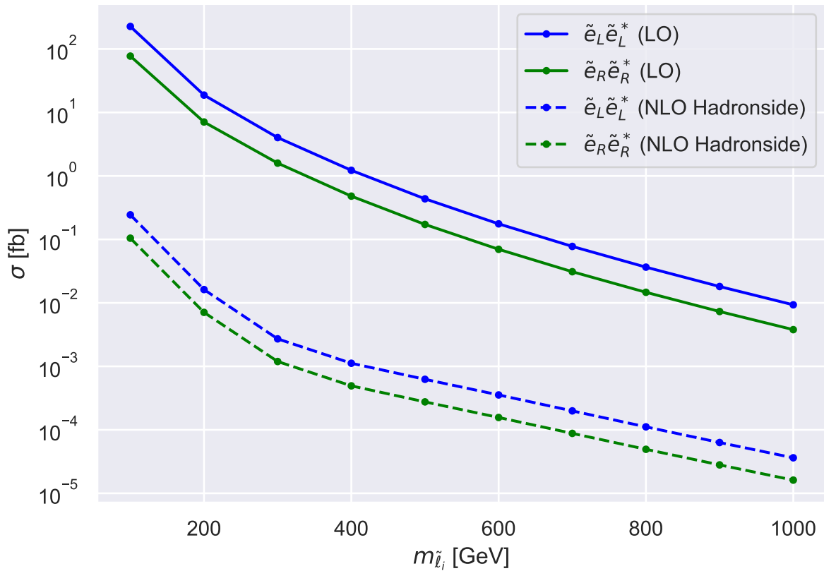
Slepton production | \sqrt{s} = 13\text{TeV}
