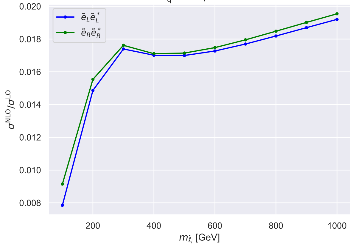
Ratio \sigma_q^{\text{NLO}}/\sigma^{\text{LO}} \mid \sqrt{s} = 13\text{TeV}
