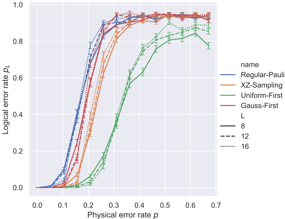
Logical error rate p_L as a function of physical error rate p .
