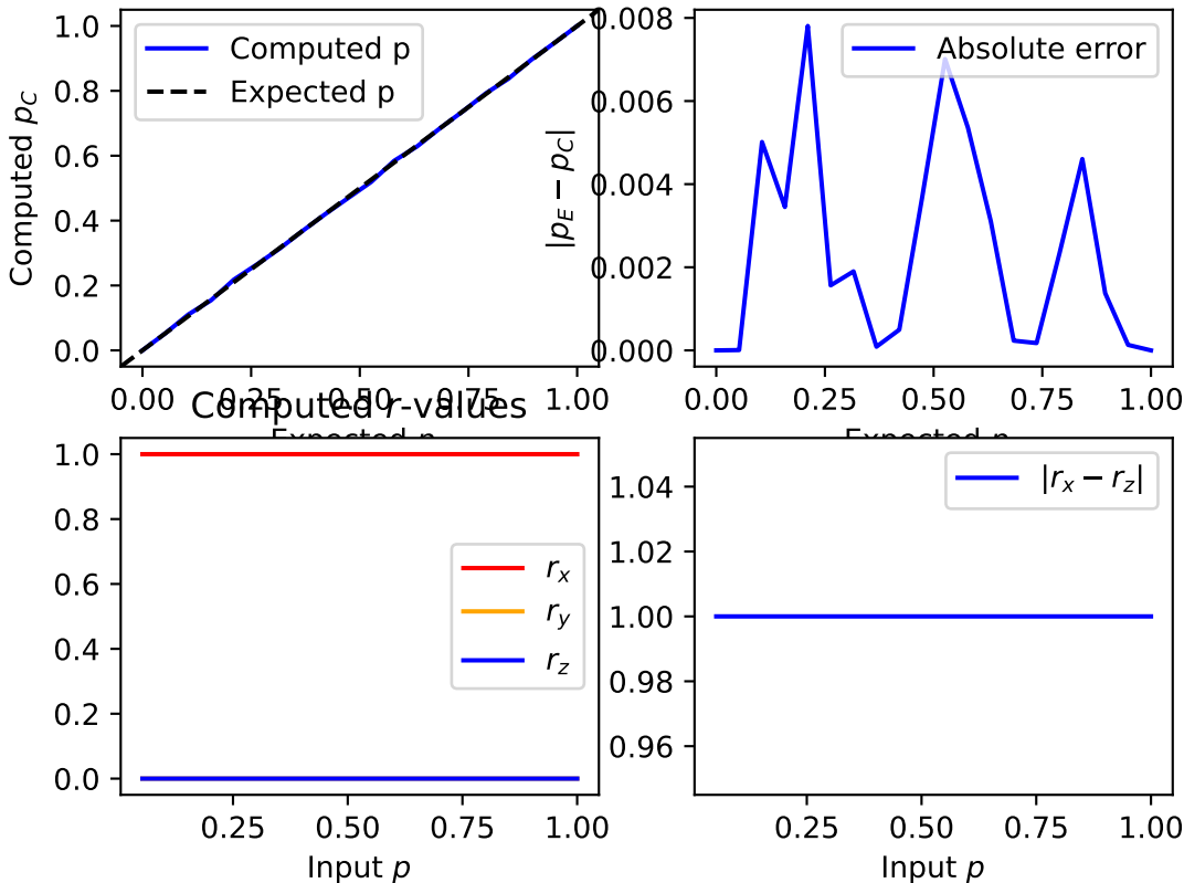
Computed error rates p from Gaussian PauliErrorModel
