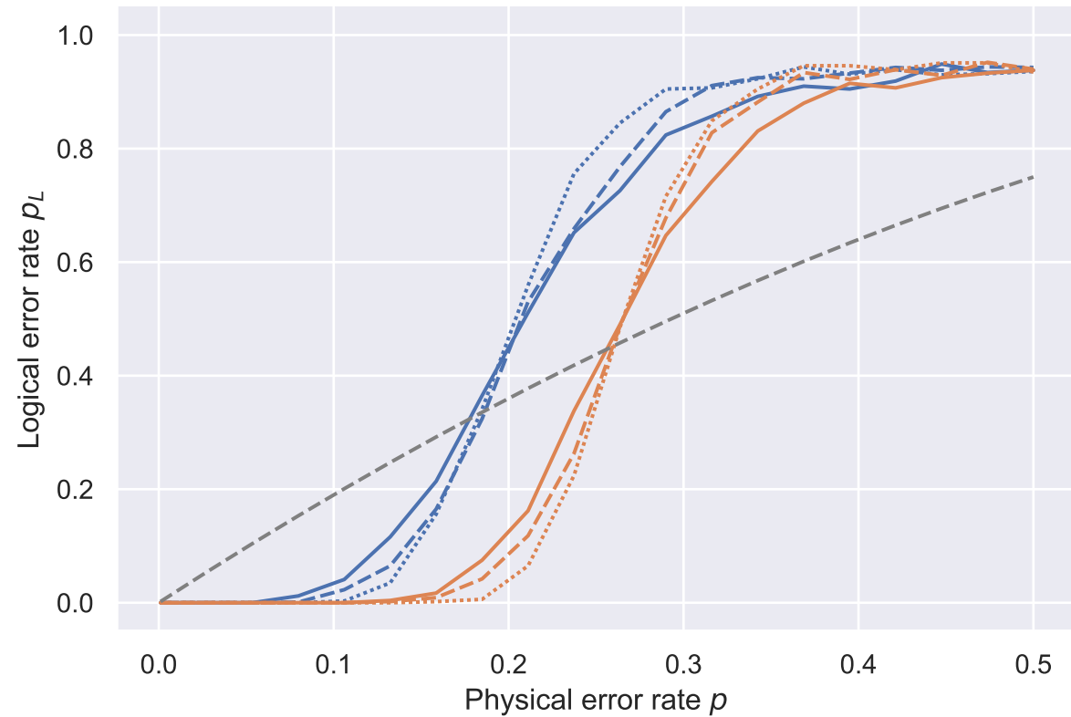
code = Toric2DCode
