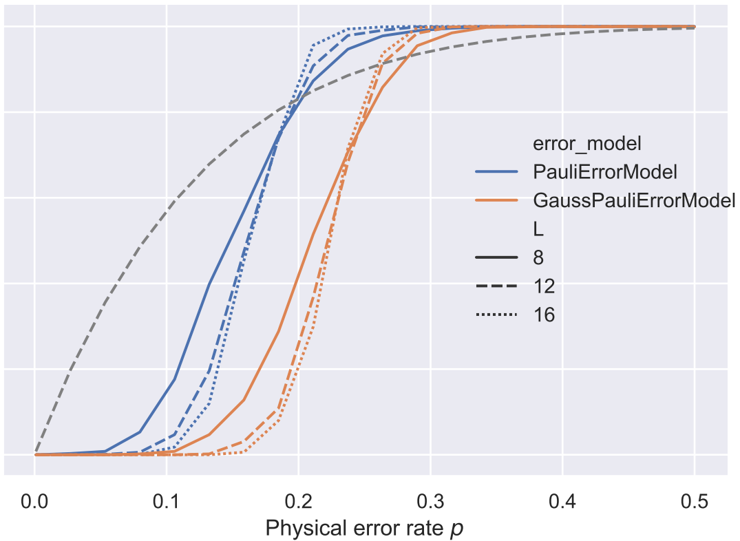
code = TileCode_B3_W6
