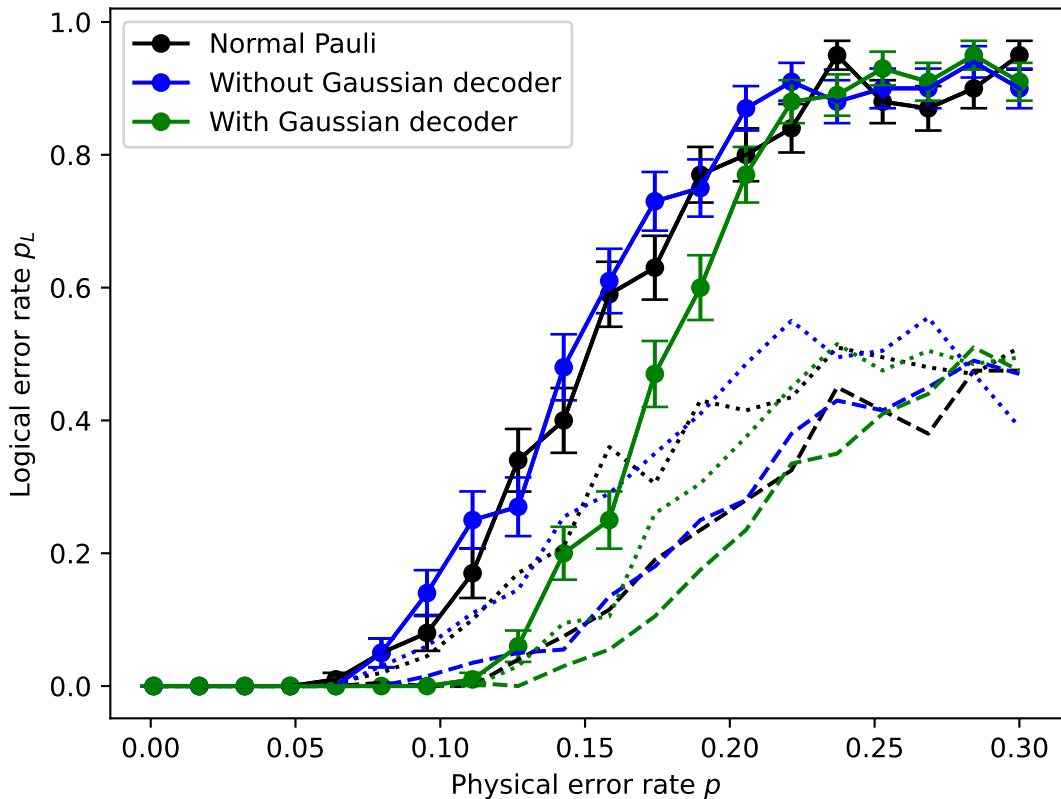
Logical error rate for X (dashed), Z (dotted), and combined (solid) sector.
