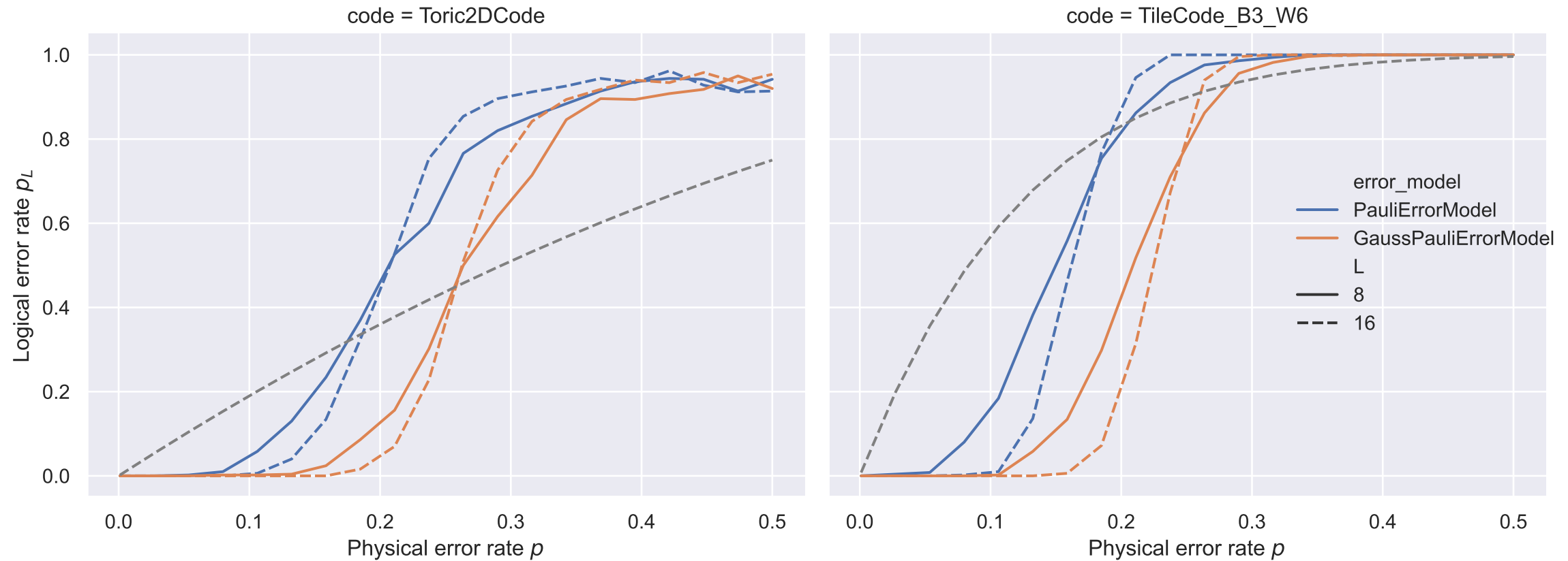
Logical error rate p_L as a function of physical error rate p . (Pseudo threshold in gray)
