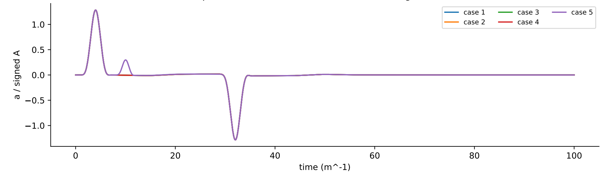
Amplitude-normalized incident and returning waveform
