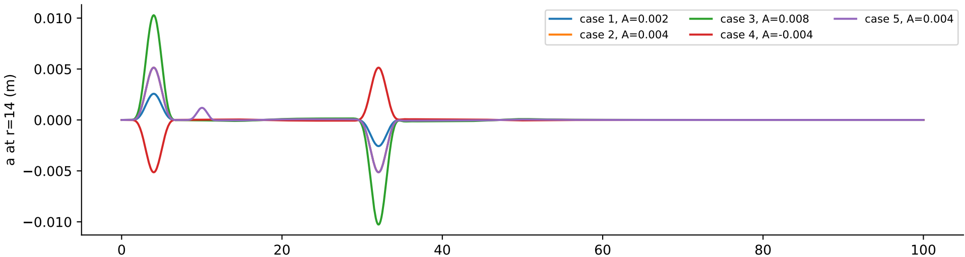
Amplitude-normalized incident and returning waveform
