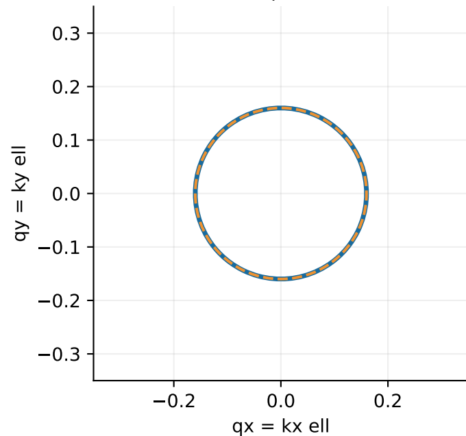
Orthogonal | Gram rank 3
