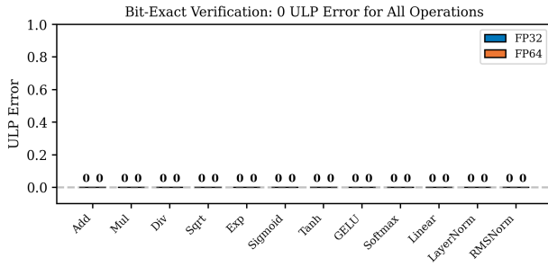
Figure 1. Bit-exact verification showing 0 ULP error (matching IEEE 754 machine precision) for all arithmetic and activation operations across FP32 and FP64 precisions.
