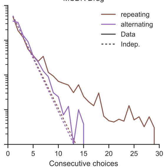
MCDR Drug
