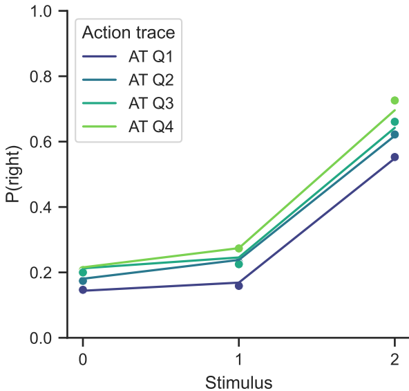
MCDR
