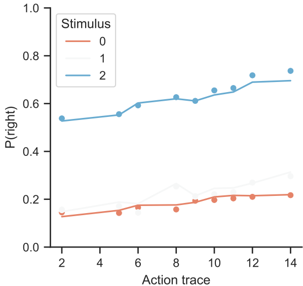
MCDR
