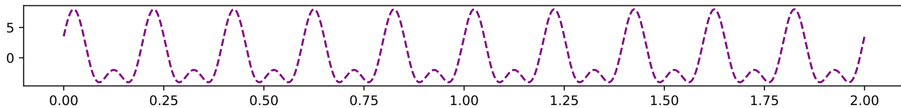
Noise
