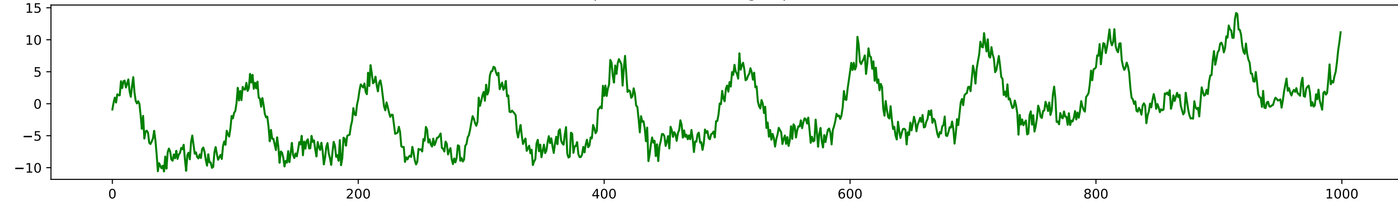
Triple Exponential Smoothing (alpha=0.7, beta=0.5, gamma=0.3)
