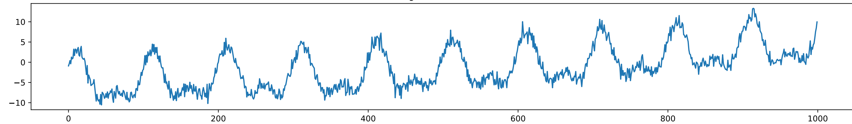
Simple Exponential Smoothing (best alpha=1.00)
