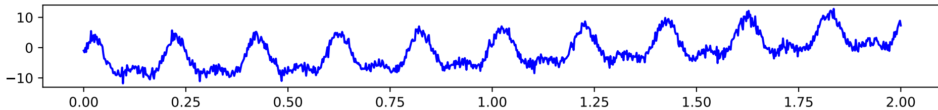
Time Series
