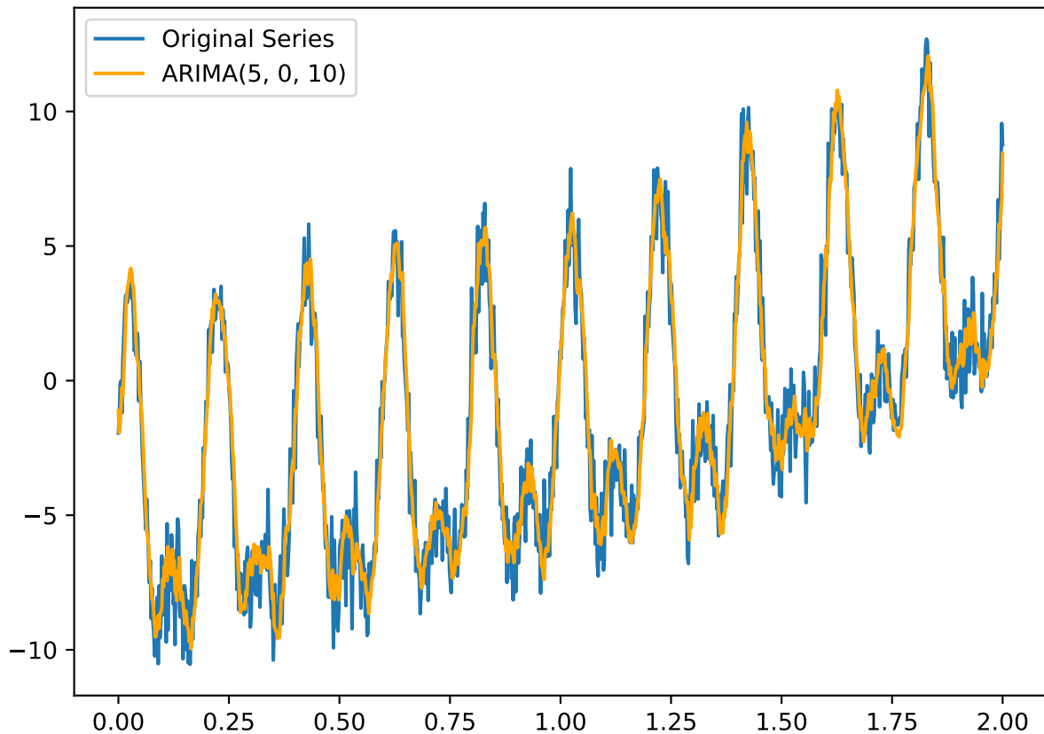
Best ARIMA Model: ARIMA(5, 0, 10)
