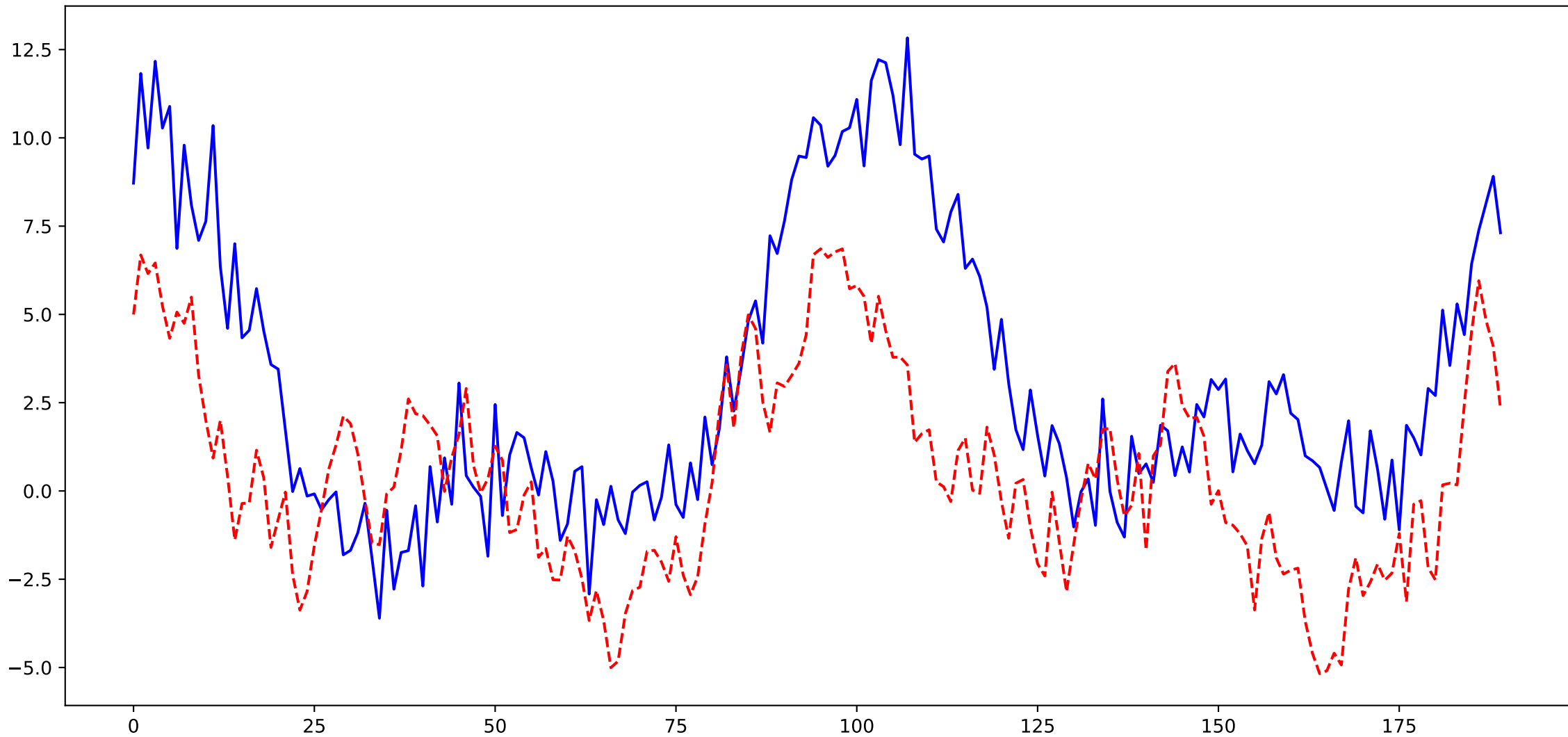
Sparse AR Model Predictions (Greedy Selection)
