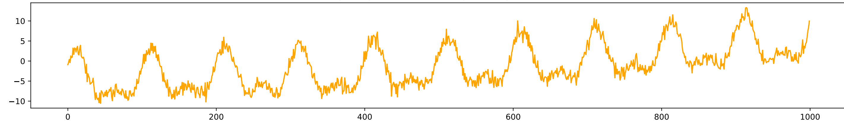
Double Exponential Smoothing (best alpha=1.00, best beta=0.10)
