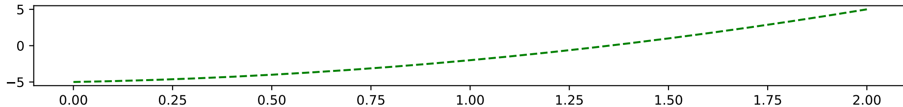
Seasonal
