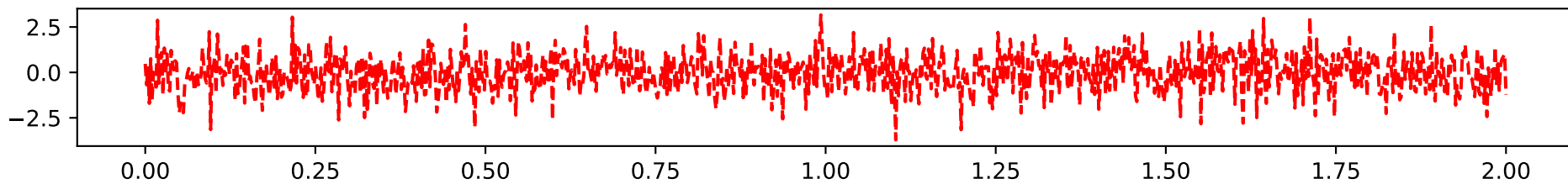
Time Series
