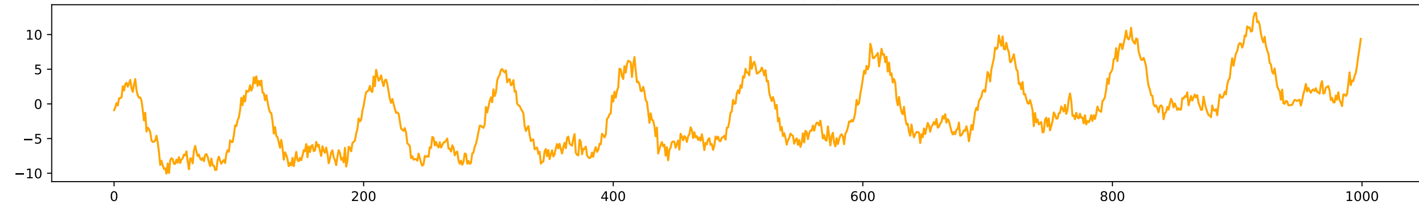
Double Exponential Smoothing (alpha=0.7, beta=0.5)
