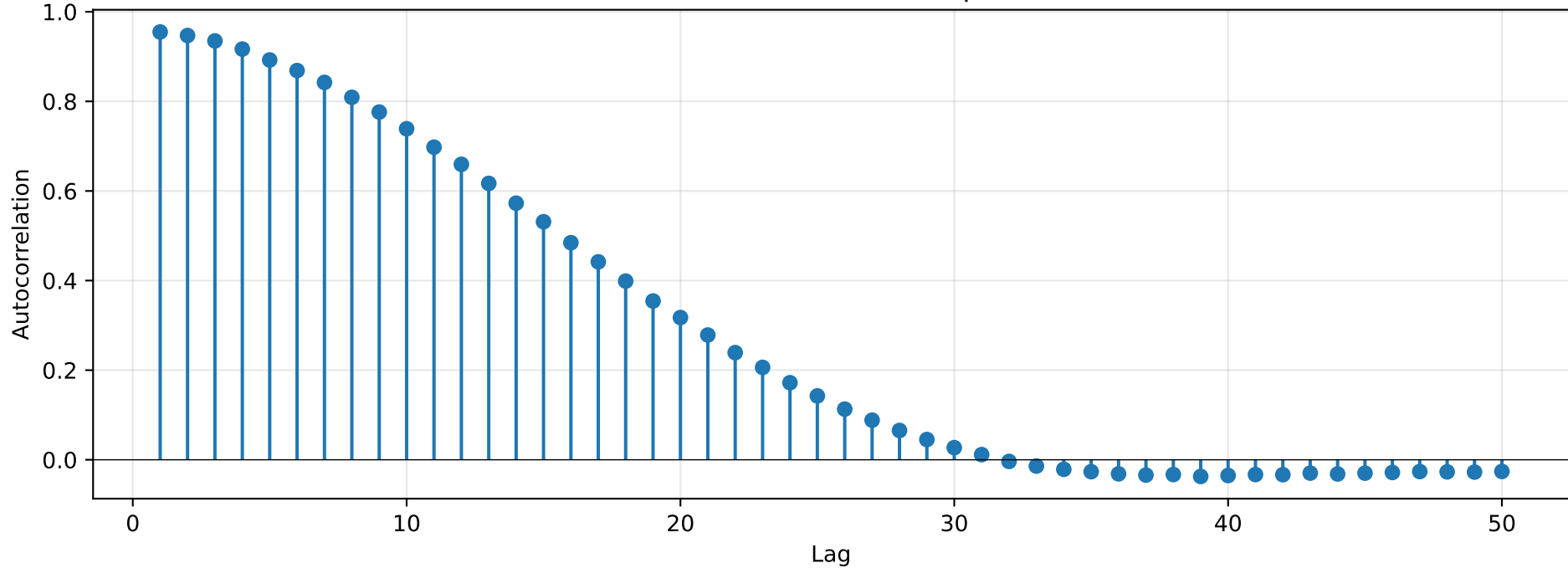
Autocorrelation Function (p=50)
