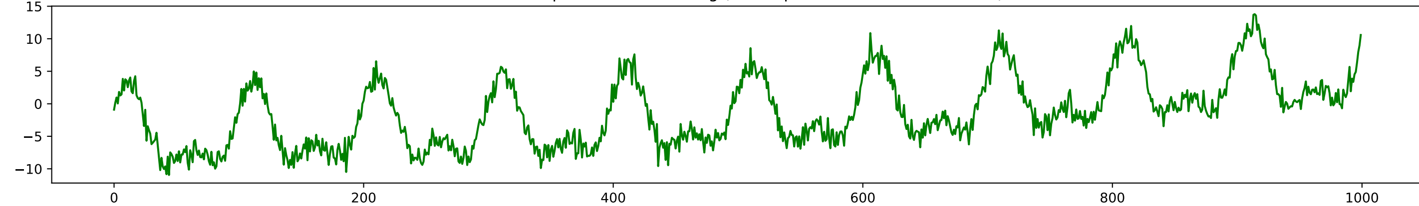
Triple Exponential Smoothing (best alpha=0.60, best beta=0.20, best gamma=0.80)
