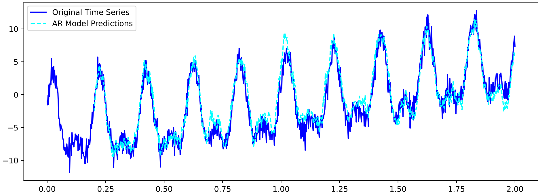
AR Model Predictions vs Original Time Series
