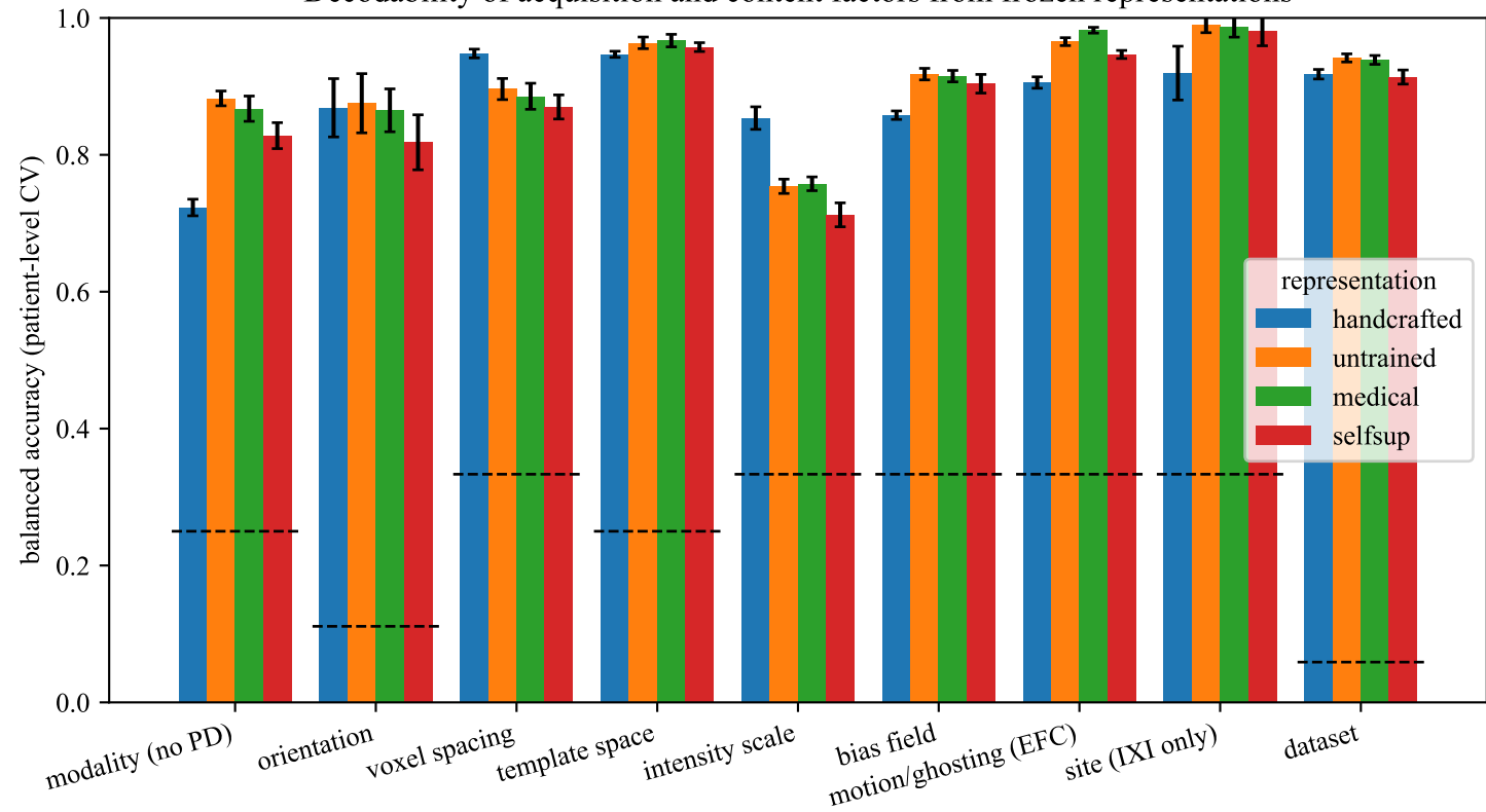
Decodability of acquisition and content factors from frozen representations
