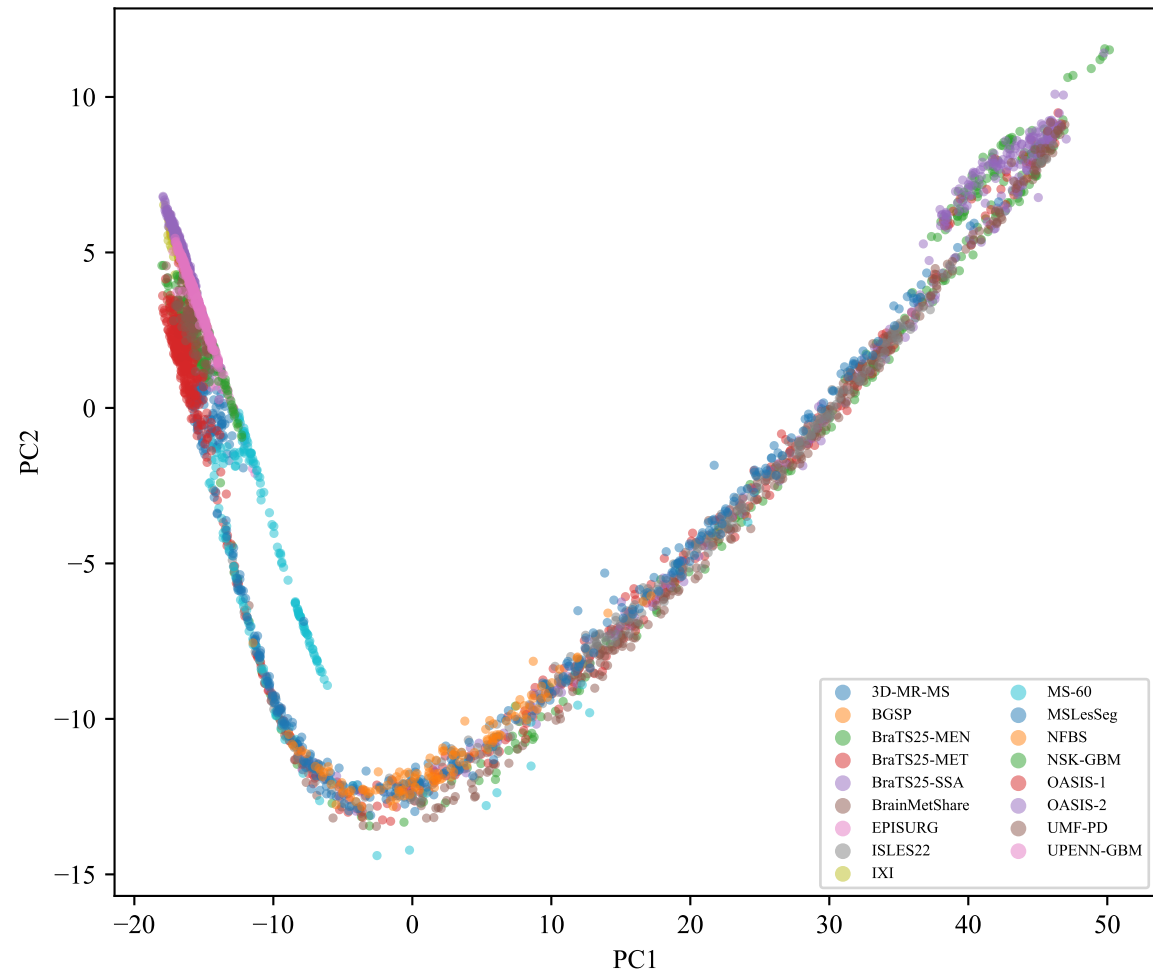
R3 embeddings — PCA(2)
