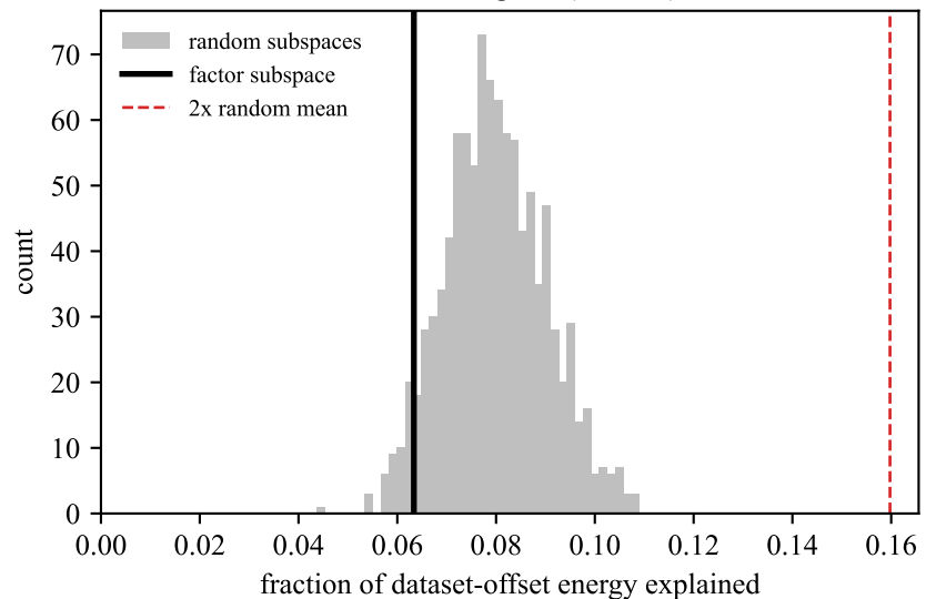
medical: signal (Gate 2)
