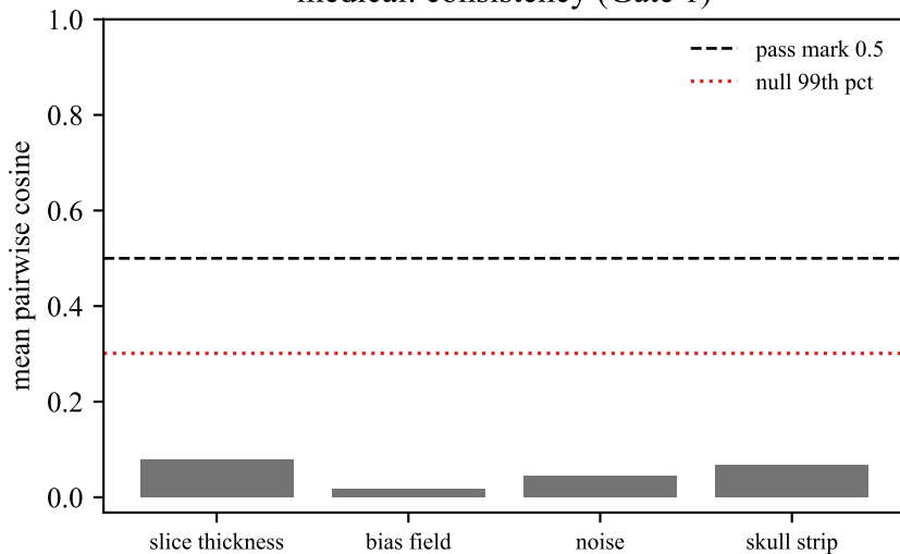
medical: consistency (Gate 1)
