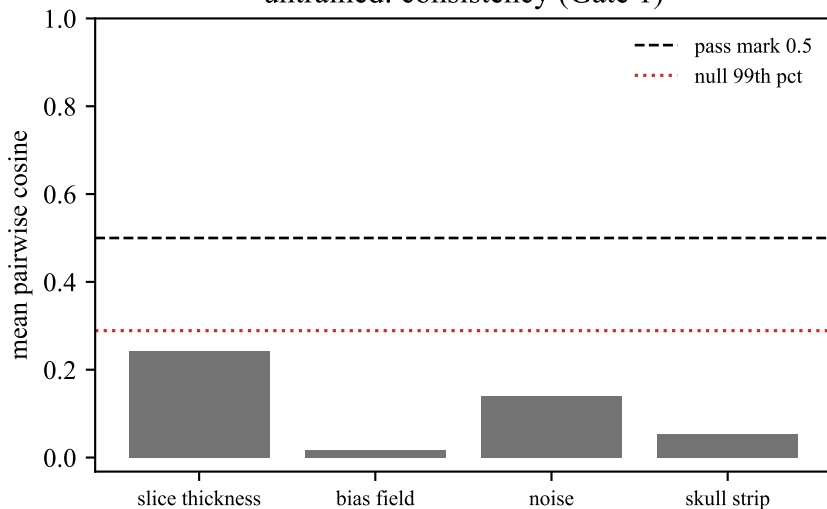
untrained: consistency (Gate 1)
