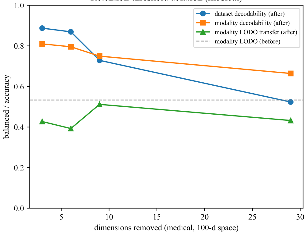
Retention-threshold ablation (medical)
