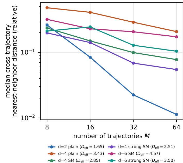
(A) Overlap availability scales with the effective dimension
