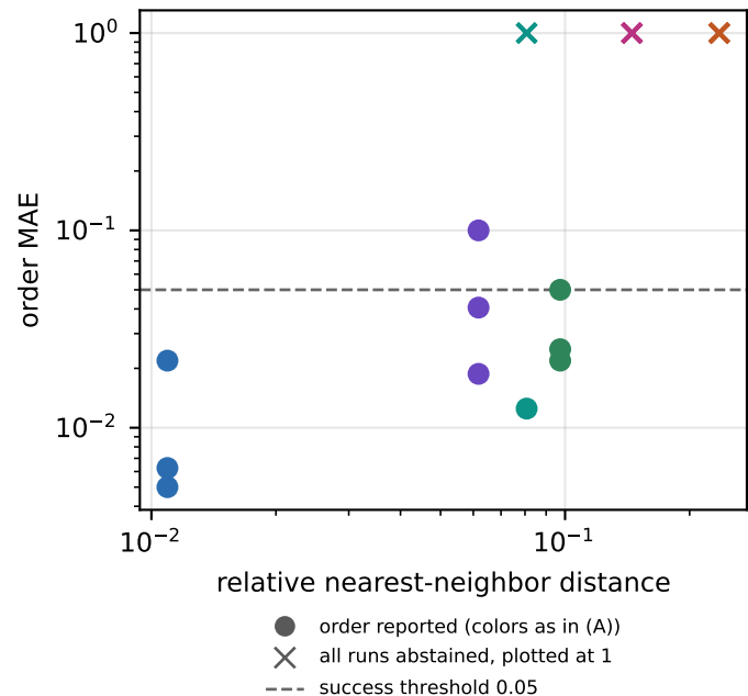
(C) Accuracy tracks overlap availability, not the state dimension
