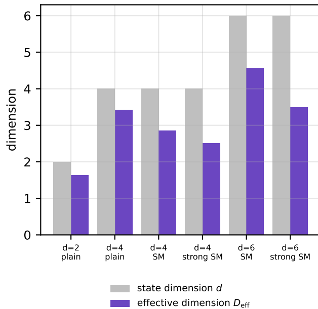
(B) Dissipation lowers the effective dimension
