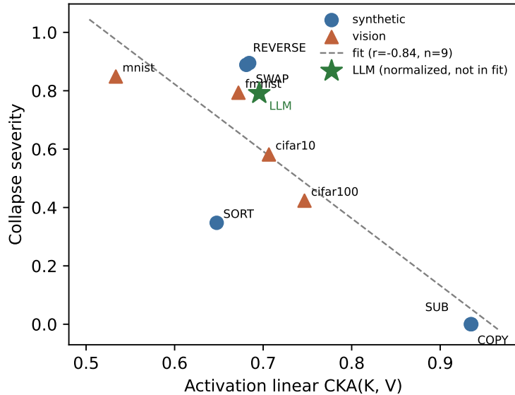
Figure 4: Activation-level linear CKA between a teacher’s trained K and V projections vs. the accuracy drop under K=V surgery (averaged over KEEP_K and KEEP_V ), across all 5 synthetic tasks and 4 vision datasets. Pearson r = -0.84 ( n = 9 ); see text for why we do not treat this as a validated general predictor. The star marks the same measurement on the 300M-parameter FineWeb-Edu teacher (CKA = 0.70), with its y -coordinate a chance-normalized log-loss severity in place of accuracy drop (Table 4 only gives perplexity, which has no shared scale with accuracy): (\ell_{\text{surgery}} - \ell_{\text{teacher}}) / (\ln |V| - \ell_{\text{teacher}}) , where \ell = \ln(\text{PPL}) and \ln |V| is the cross-entropy of a uniform predictor over the vocabulary – the LM analogue of chance accuracy. Excluded from the fit regardless, since this is a different derivation from the other 9 points’ raw accuracy drop, not a directly validated equivalent measure.
