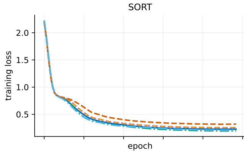
Synthetic-task training loss (d=64, L=2, H=4, T=64; mean of 3 seeds)
