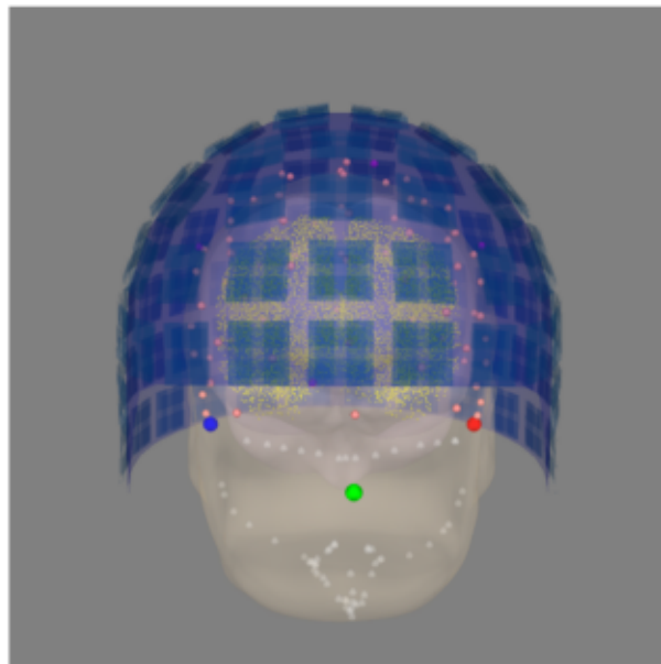
sub010 (our S09): coregistration front
