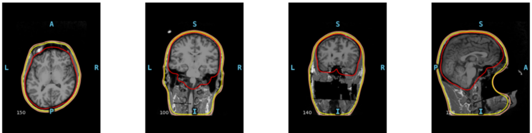
our reproduction sub004 (paper subject 4): watershed BEM surfaces on T1
