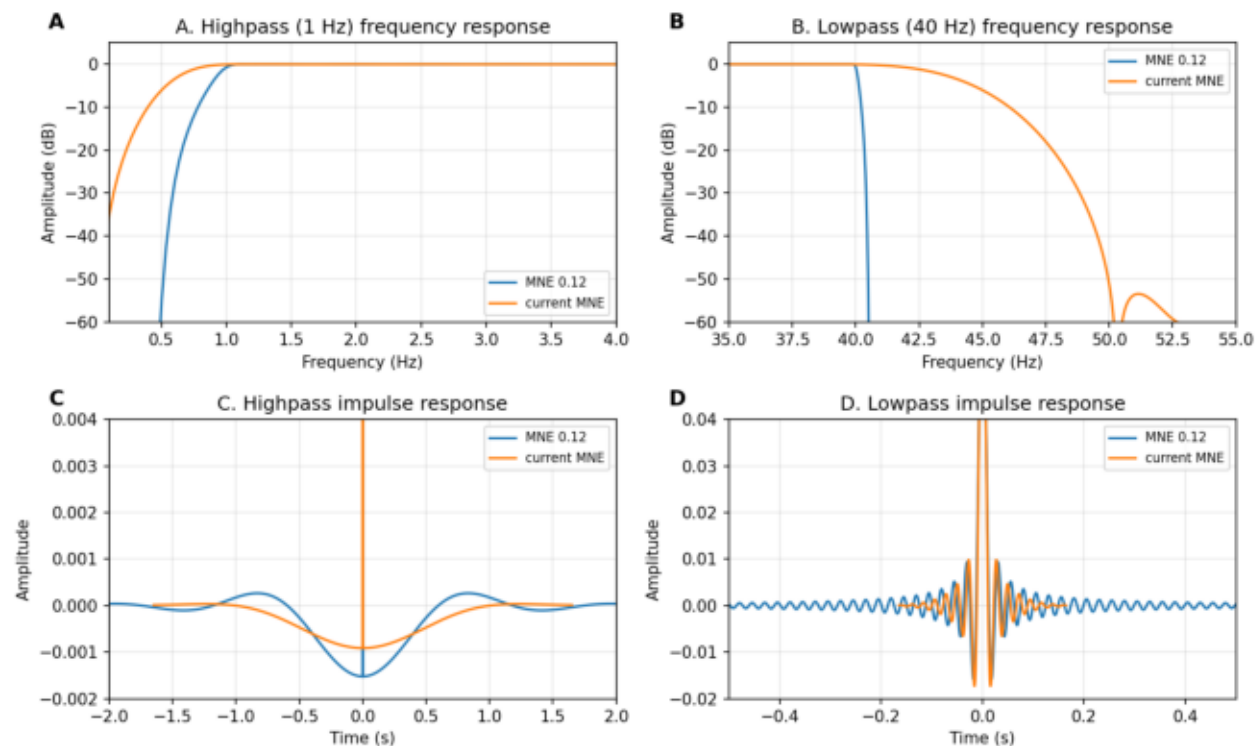
Figure 3 (reproduction) — filter response, MNE 0.12 vs. current MNE 1.12.1
