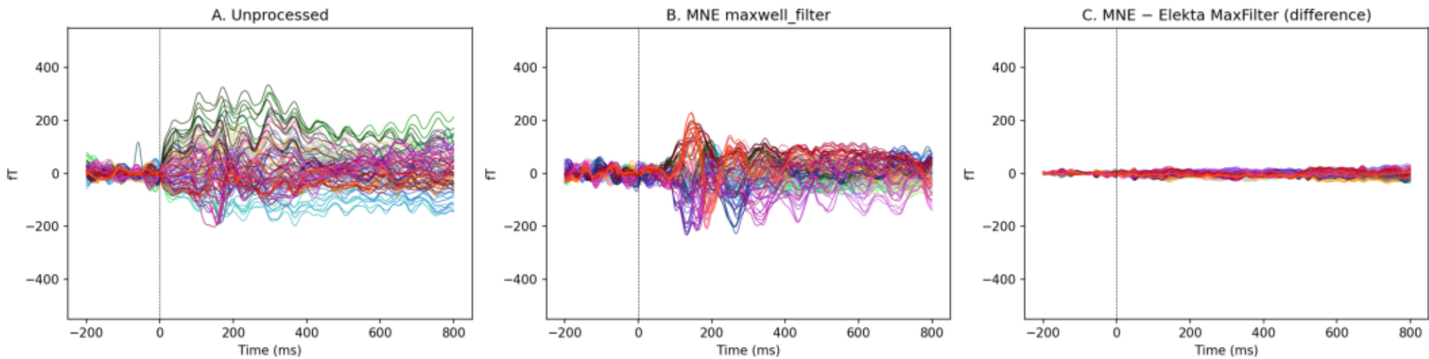
Figure 1 (reproduction) — Subject 09, Run 02 — magnetometers, 1-40 Hz
