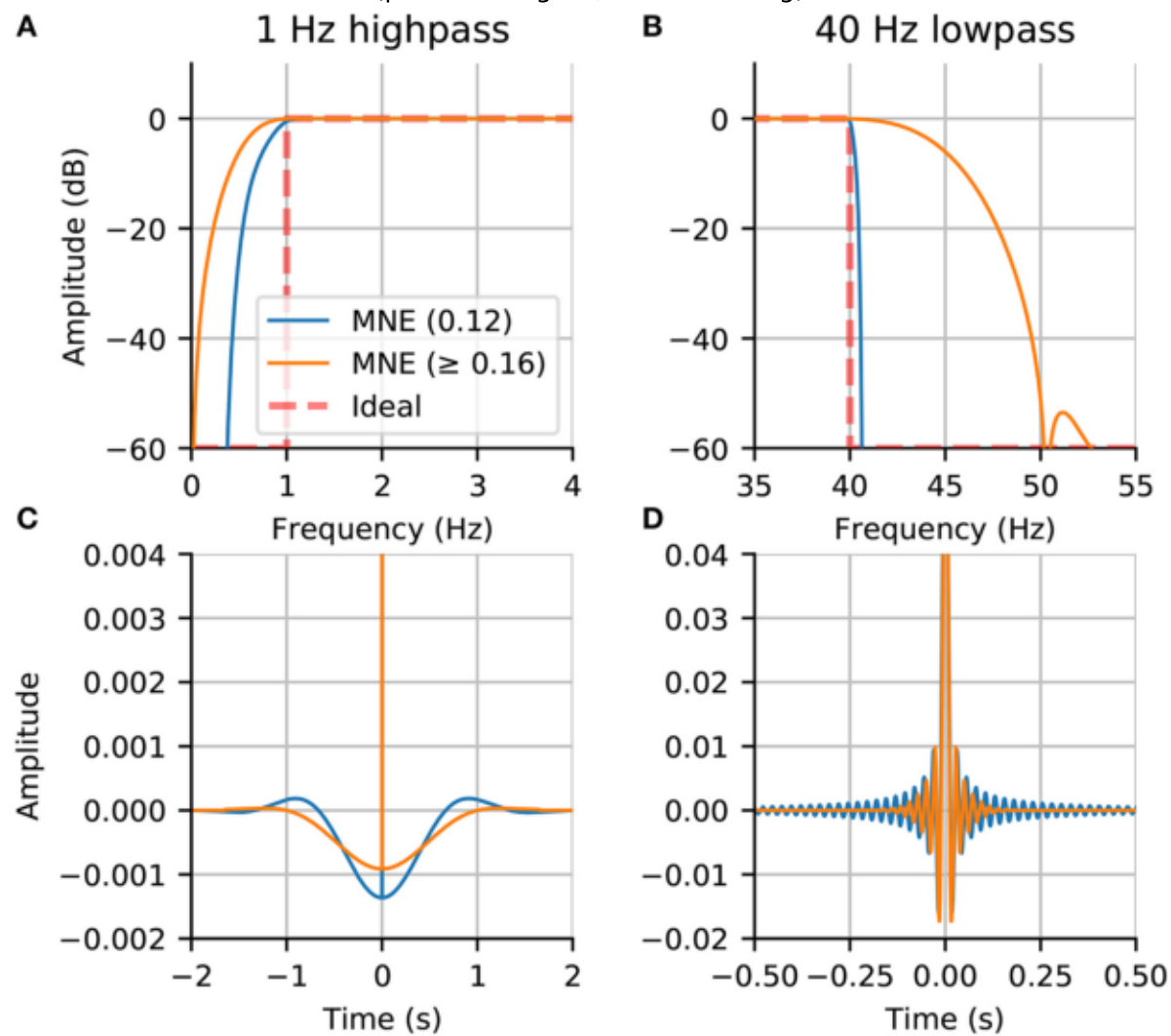
Figure 3 (reproduction) — filter response, MNE 0.12 vs. current MNE 1.12.1
