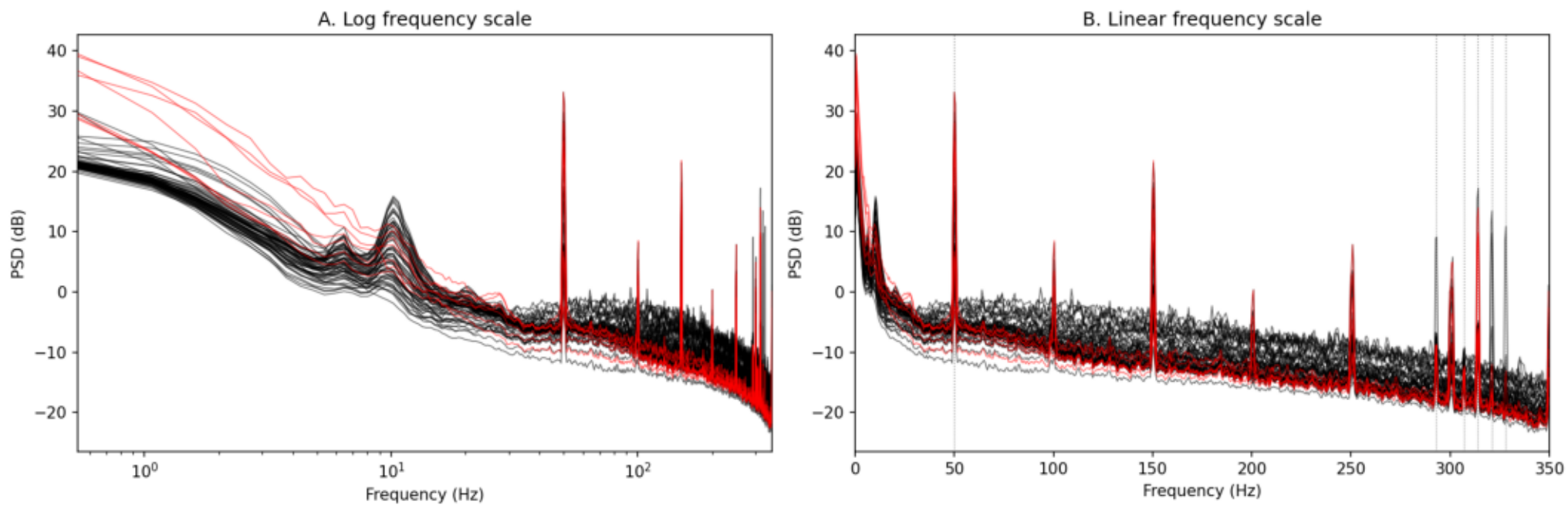
Figure 2 (reproduction) — Subject 09, Run 02 — EEG channel PSD (raw, pre-SSS)
