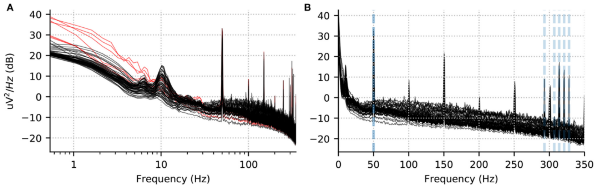
Jas et al. 2018, Figure 2 -- PSD quality control (published figure, frontiersin.org)
