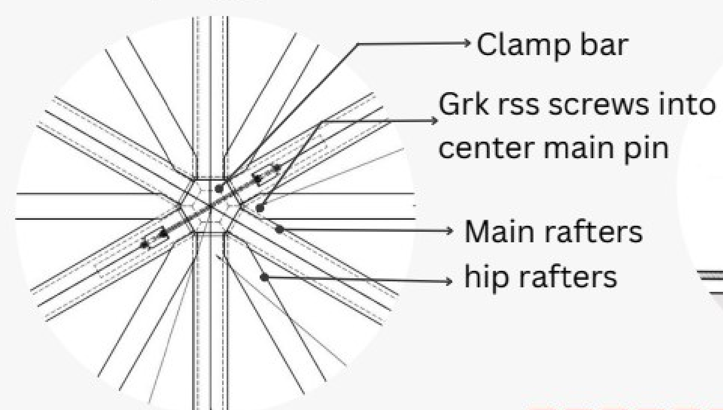
Timber frame connection detail of the polygonal dome
