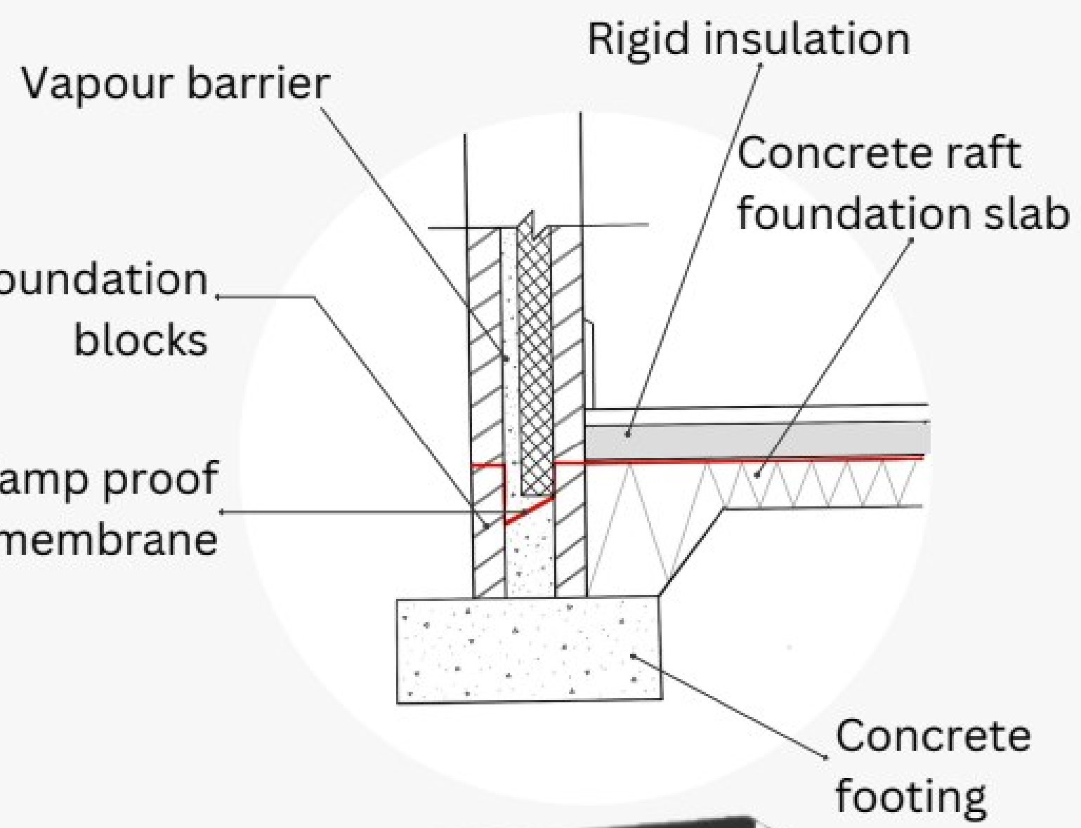
Foundation detail
