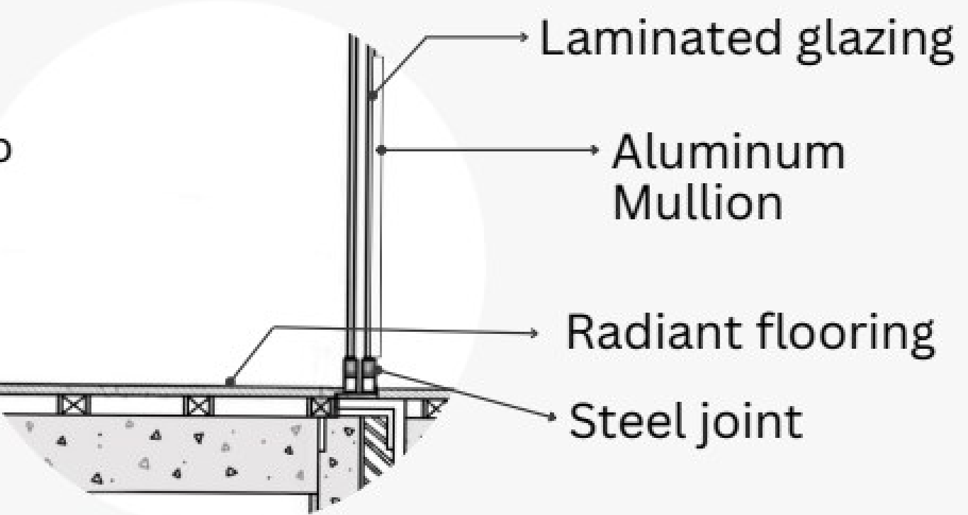
Curtain wall sectional detail
