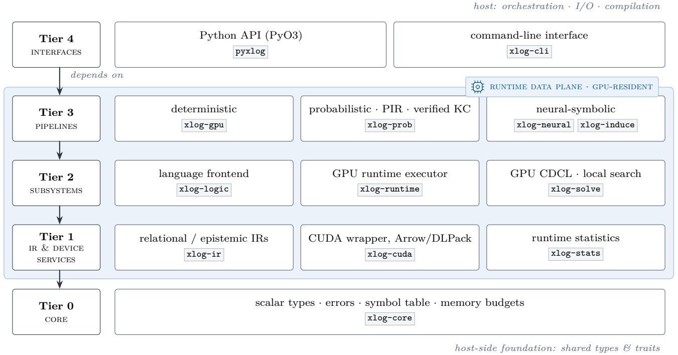
Figure 1: xlog crate hierarchy. Each tier depends only on lower tiers; the shaded device plane marks GPU-resident runtime data planes, while the host provides orchestration, I/O, compilation, and bounded control reads.
