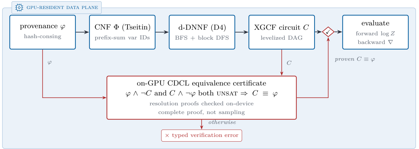
Figure 2: Verified knowledge-compilation pipeline. The data plane uses CUDA kernels and device-resident state under host orchestration. The final smoothed circuit C reaches evaluation only through the equivalence gate ( \checkmark ): an on-GPU CDCL solver proves \varphi \wedge \neg C and C \wedge \neg \varphi both unsatisfiable; the host observes bounded status and error scalars, and any failed or incomplete proof returns a typed error.
